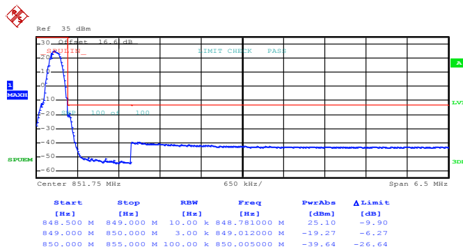
Higher Band Edge Plot on Channel 251 (848.8 MHz)
