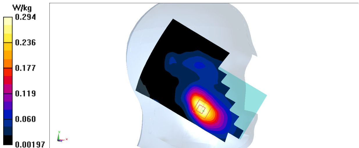
Fig.9 LTE Band2
