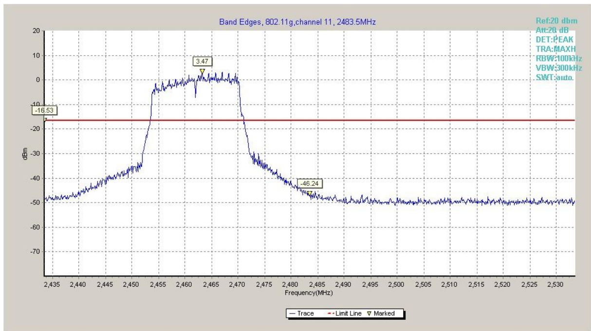
Fig.A.5.6 Band Edges (802.11g, Ch 11)
