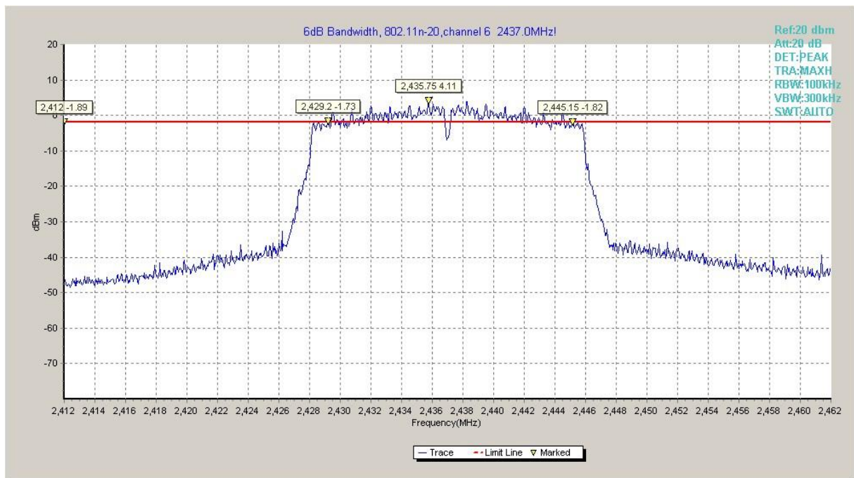
Fig.A.4.12 Occupied 6dB Bandwidth (802.11n-HT20, Ch 6)
