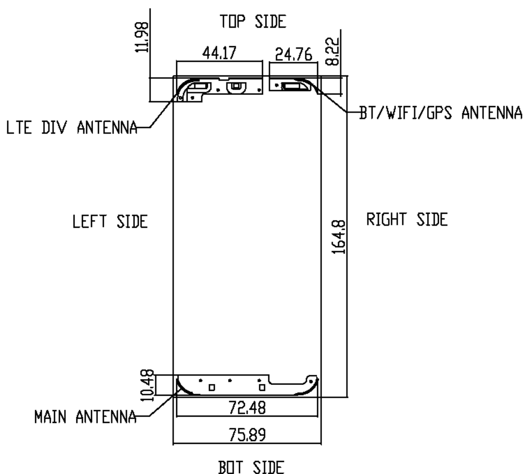
Picture 11.1 Antenna Locations (Front View)
