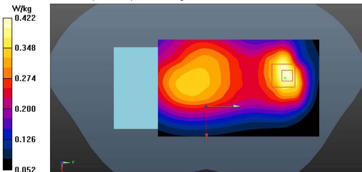
Fig.2 GSM850 Body
