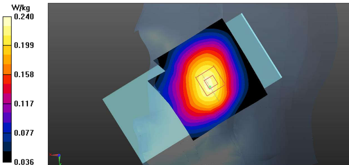
Fig.1 GSM850 Head
