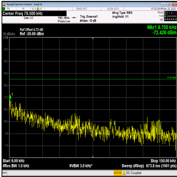
Band41_10MHz_16QAM_40090_1RB#0_0.009~0.15_0.009~0.15
