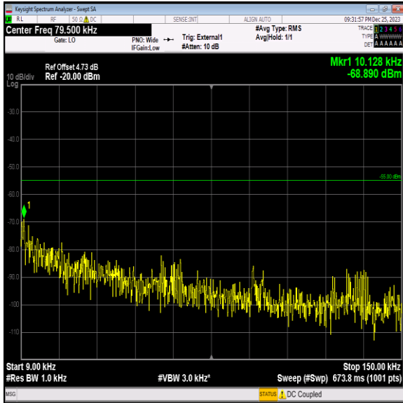
Band41_15MHz_64QAM_41165_1RB#0_0.009~0.15_0.009~0.15
