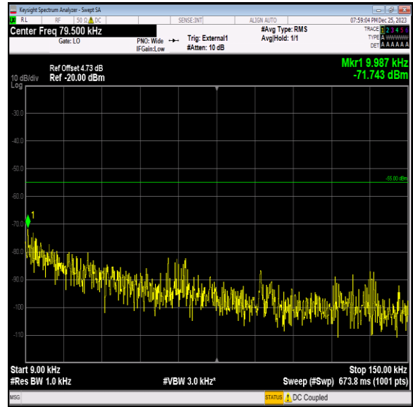
Band41_10MHz_16QAM_40640_1RB#0_0.009~0.15_0.009~ 0.15
