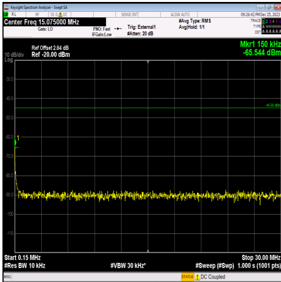
Band41_15MHz_64QAM_40640_1RB#0_0.15~30_0.15~30
