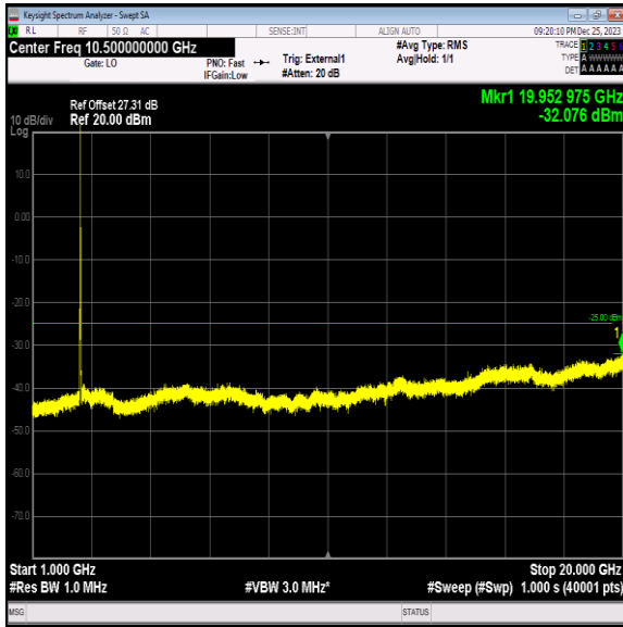
Band41_15MHz_16QAM_40115_1RB#0_1000~20000_1000~20000
