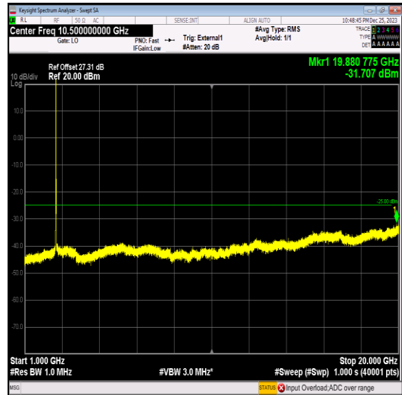
Band41_20MHz_QPSK_40640_1RB#0_1000~20000_1000~20000
