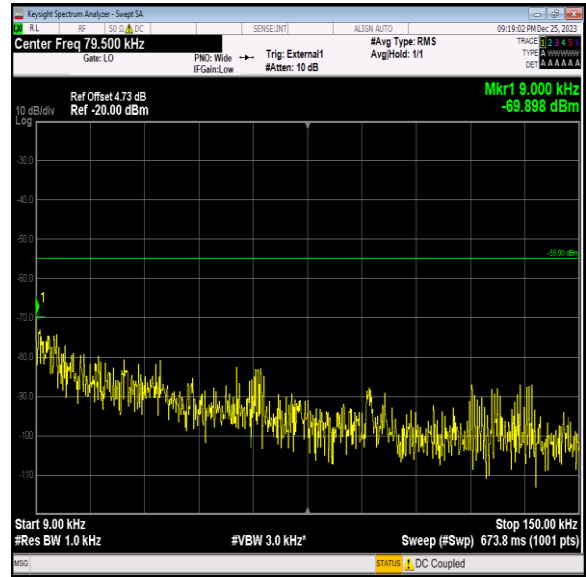
Band41_15MHz_16QAM_40115_1RB#0_0.009~0.15_0.009~0.15
