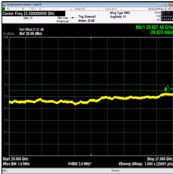
Band41_15MHz_64QAM_41165_1RB#0_20000~27000_20000~27000
