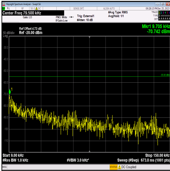
Band41_15MHz_QPSK_41165_1RB#0_0.009~0.15_0.009~0.15
