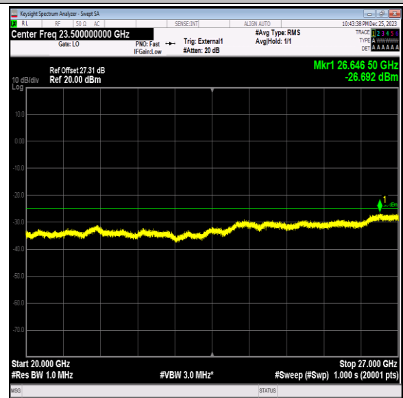
Band41_20MHz_QPSK_40140_1RB#0_20000~27000_20000~27000
