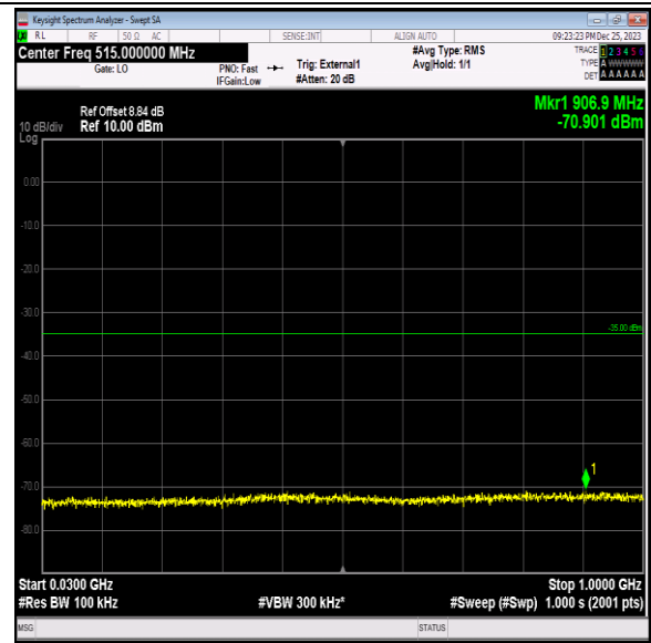
Band41_15MHz_QPSK_40640_1RB#0_30~1000_30~1000
