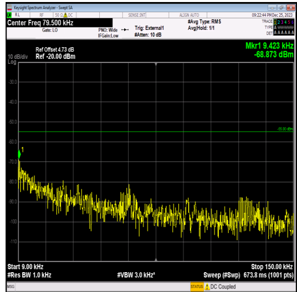
Band41_15MHz_QPSK_40640_1RB#0_0.009~0.15_0.009~0.15
