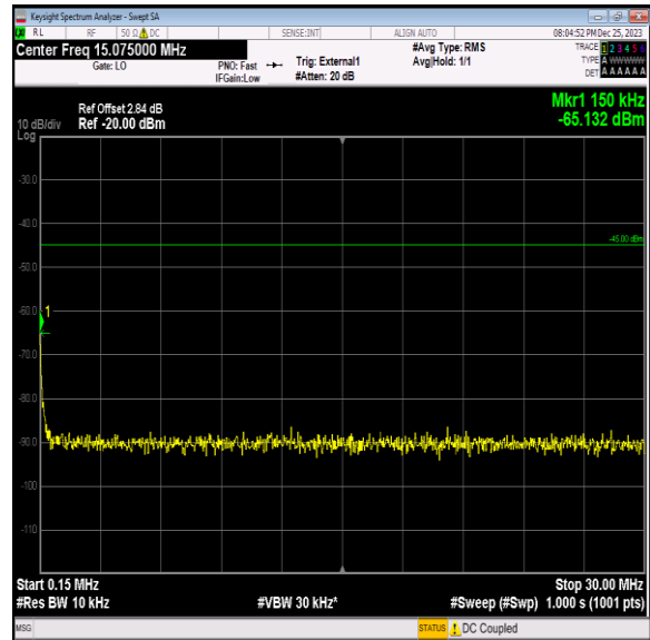
Band41_10MHz_16QAM_41190_1RB#0_0.15~30_0.15~30
