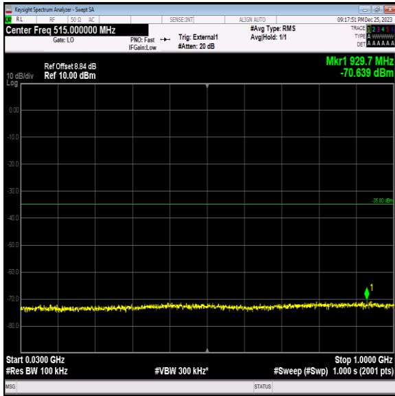
Band41_15MHz_QPSK_40115_1RB#0_30~1000_30~1000
