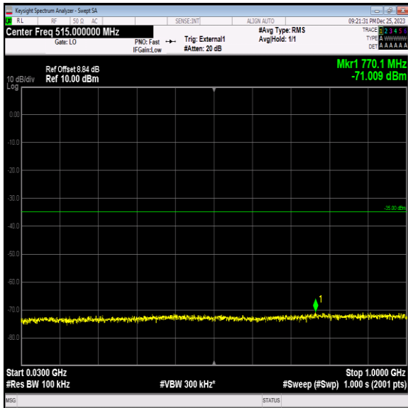
Band41_15MHz_64QAM_40115_1RB#0_30~1000_30~1000
