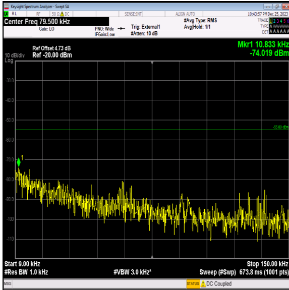
Band41_20MHz_16QAM_40140_1RB#0_0.009~0.15_0.009~0.15
