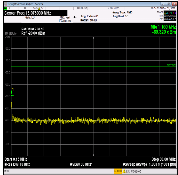
Band41_15MHz_16QAM_40640_1RB#0_0.15~30_0.15~30
