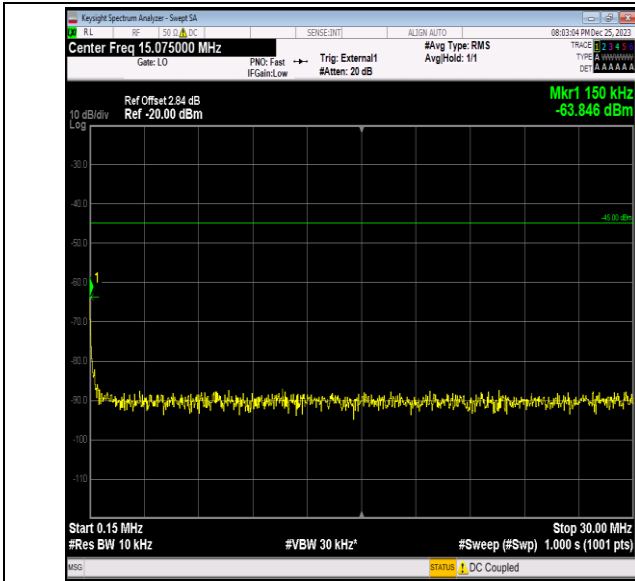
Band41_10MHz_QPSK_41190_1RB#0_0.15~30_0.15~30
