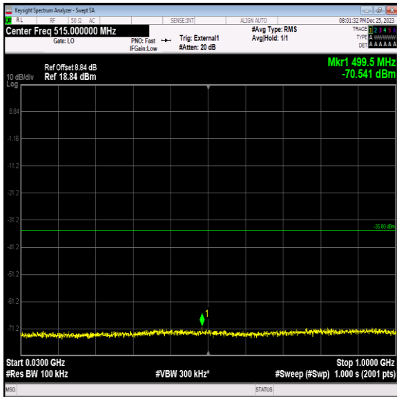
Band41_10MHz_64QAM_40640_1RB#0_30~1000_30~1000
