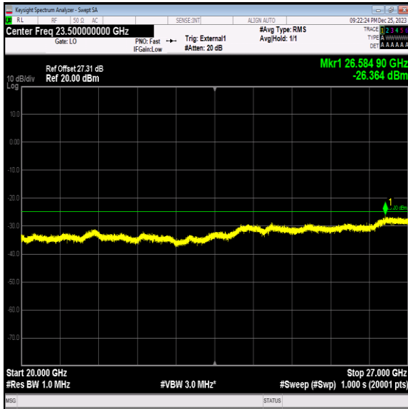
Band41_15MHz_64QAM_40115_1RB#0_20000~27000_2000 0~27000
