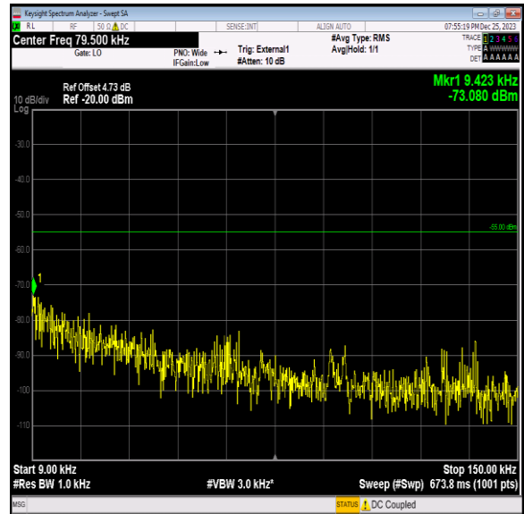
Band41_10MHz_64QAM_40090_1RB#0_0.009~0.15_0.009~0.15
