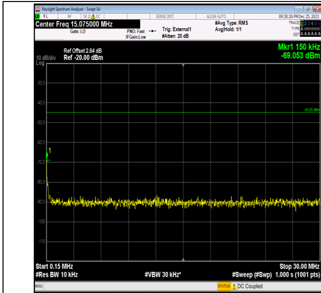
Band41_15MHz_16QAM_41165_1RB#0_0.15~30_0.15~30
