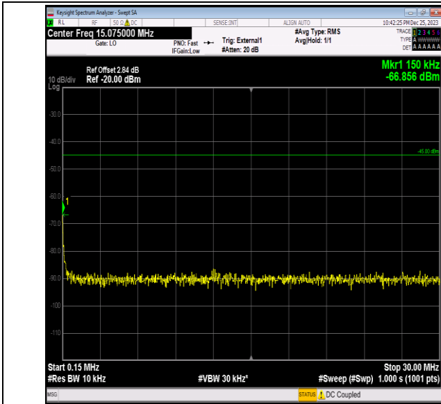
Band41_20MHz_QPSK_40140_1RB#0_0.15~30_0.15~30
