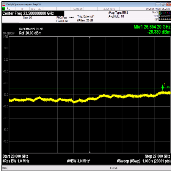
Band41_15MHz_16QAM_40640_1RB#0_20000~27000_2000~27000
