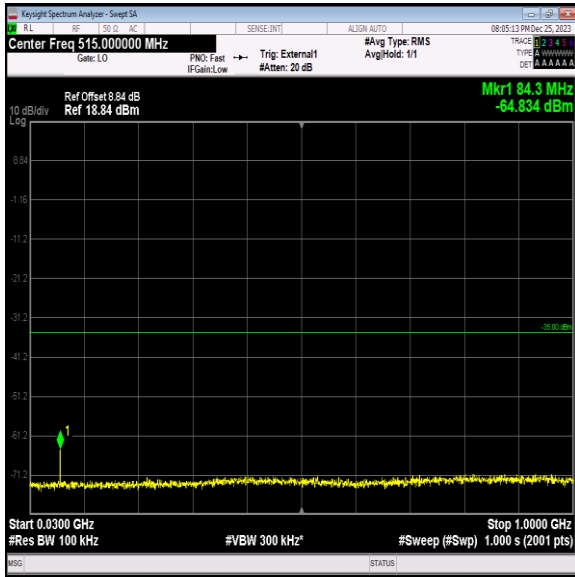
Band41_10MHz_16QAM_41190_1RB#0_30~1000_30~1000
