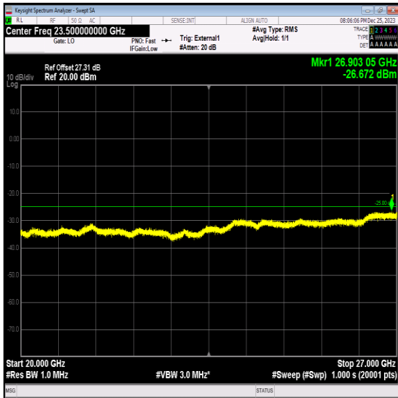
Band41_10MHz_16QAM_41190_1RB#0_20000~27000_20000~27000
