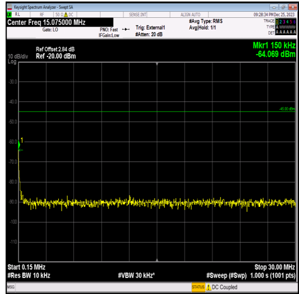
Band41_15MHz_QPSK_41165_1RB#0_0.15~30_0.15~30
