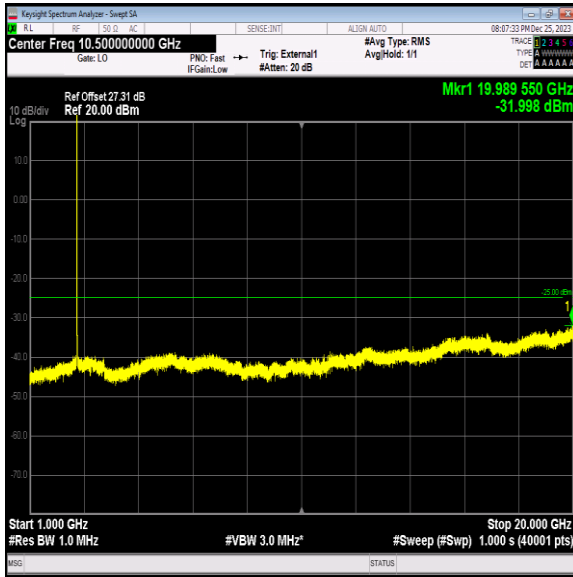
Band41_10MHz_64QAM_41190_1RB#0_1000~20000_1000~20000
