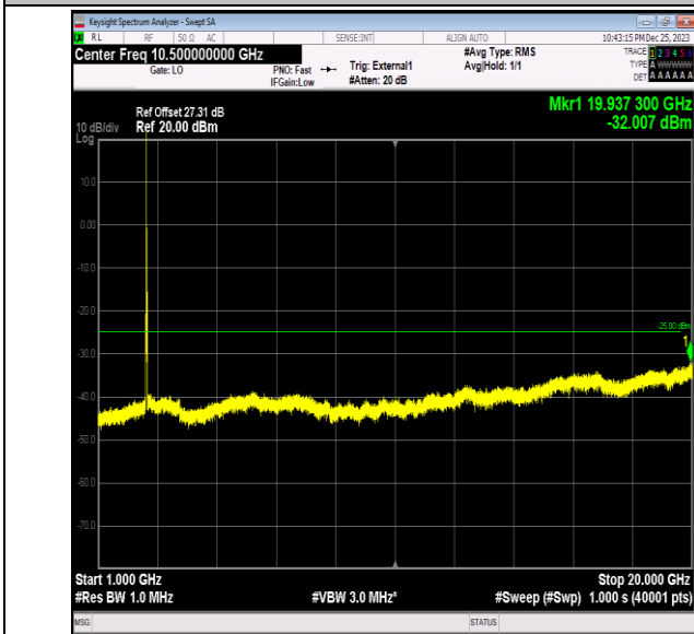
Band41_20MHz_QPSK_40140_1RB#0_1000~20000_1000~20000
