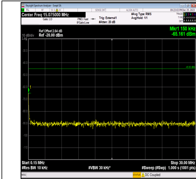
Band41_15MHz_QPSK_40640_1RB#0_0.15~30_0.15~30
