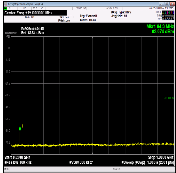
Band41_10MHz_64QAM_41190_1RB#0_30~1000_30~1000
