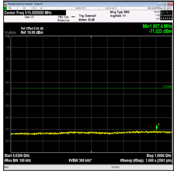
Band41_15MHz_16QAM_40115_1RB#0_30~1000_30~1000
