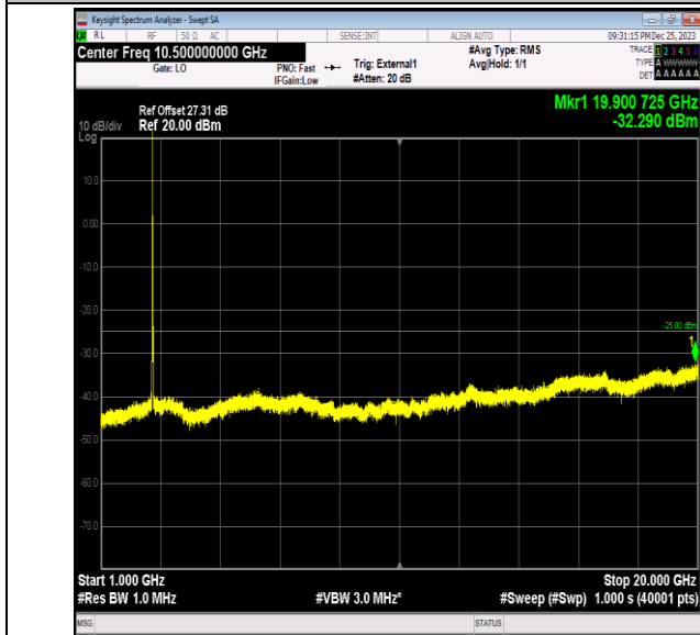
Band41_15MHz_16QAM_41165_1RB#0_1000~20000_1000~20000
