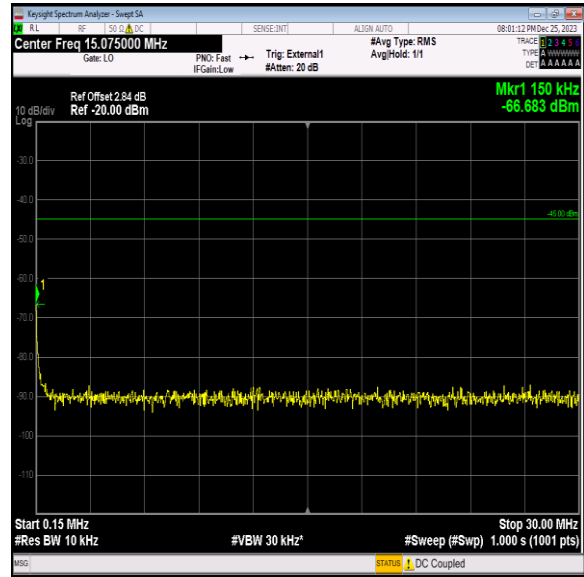
Band41_10MHz_64QAM_40640_1RB#0_0.15~30_0.15~30
