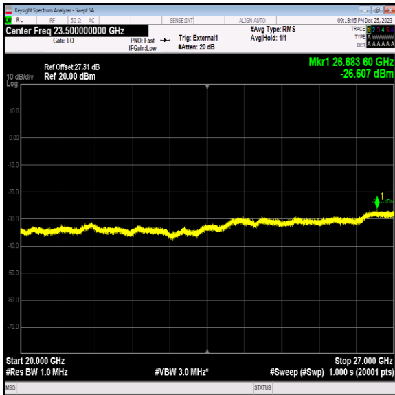
Band41_15MHz_QPSK_40115_1RB#0_20000~27000_20000~27000
