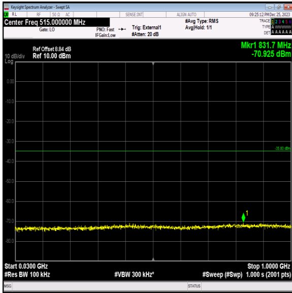
Band41_15MHz_16QAM_40640_1RB#0_30~1000_30~1000
