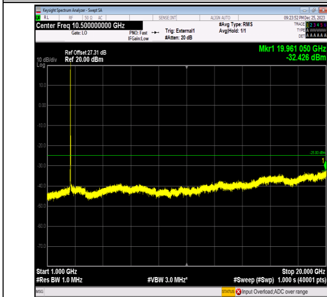
Band41_15MHz_QPSK_40640_1RB#0_1000~20000_1000~20000
