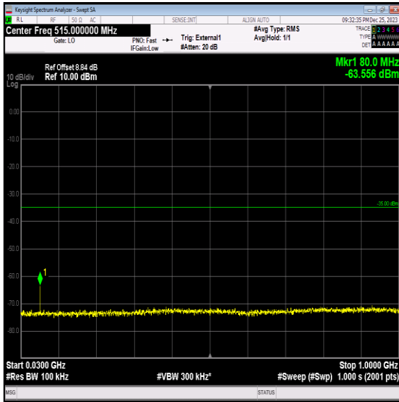
Band41_15MHz_64QAM_41165_1RB#0_30~1000_30~1000
