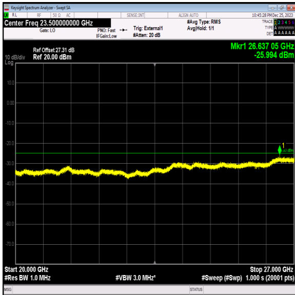
Band41_20MHz_16QAM_40140_1RB#0_20000~27000_20000~27000
