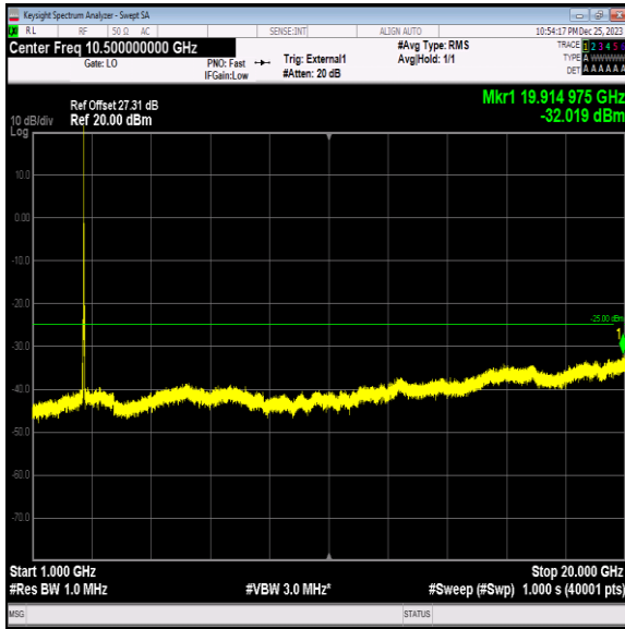
Band41_20MHz_QPSK_41140_1RB#0_1000~20000_1000~20000
