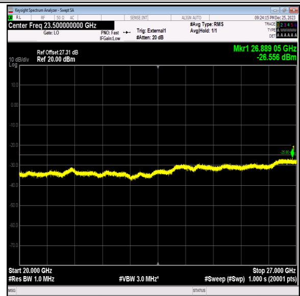
Band41_15MHz_QPSK_40640_1RB#0_20000~27000_20000~27000
