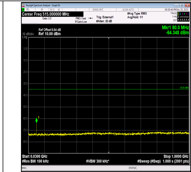
Band41_15MHz_16QAM_41165_1RB#0_30~1000_30~1000
