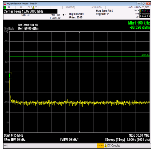
Band41_15MHz_64QAM_40115_1RB#0_0.15~30_0.15~30
