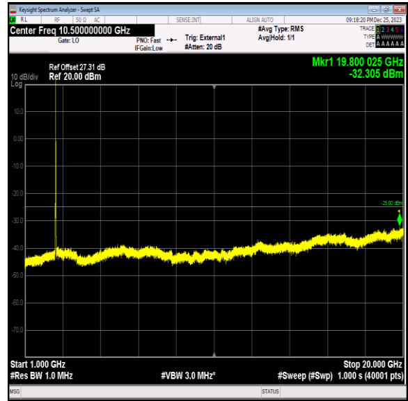
Band41_15MHz_QPSK_40115_1RB#0_1000~20000_1000~20000
