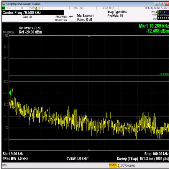
Band41_15MHz_QPSK_40115_1RB#0_0.009~0.15_0.009~0.15
