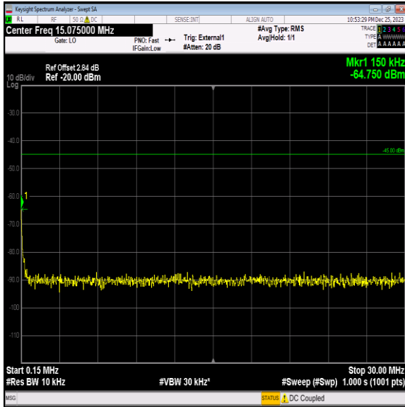
Band41_20MHz_QPSK_41140_1RB#0_0.15~30_0.15~30
