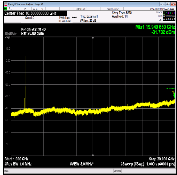
Band41_15MHz_64QAM_41165_1RB#0_1000~20000_1000~20000
