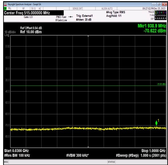
Band41_15MHz_64QAM_40640_1RB#0_30~1000_30~1000
