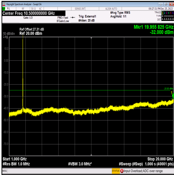
Band41_15MHz_64QAM_40640_1RB#0_1000~20000_1000~20000
