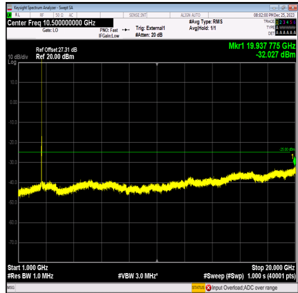
Band41_10MHz_64QAM_40640_1RB#0_1000~20000_1000~20000
