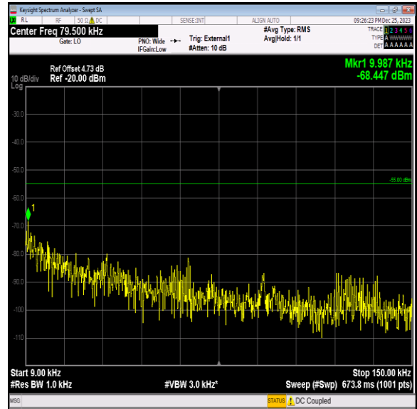
Band41_15MHz_64QAM_40640_1RB#0_0.009~0.15_0.009~ 0.15
