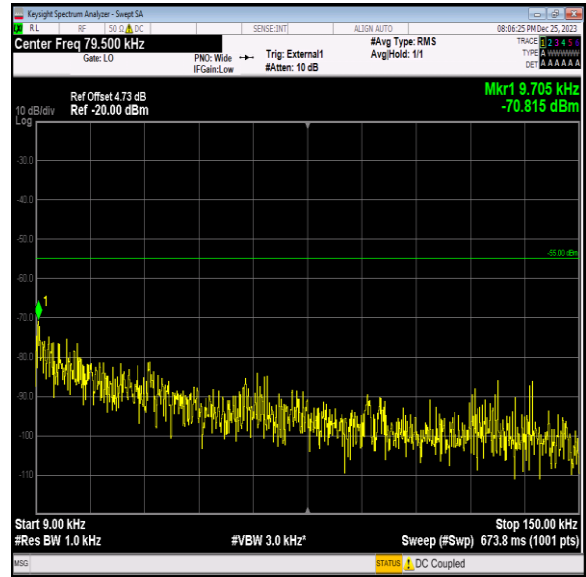
Band41_10MHz_64QAM_41190_1RB#0_0.009~0.15_0.009~0 .15
