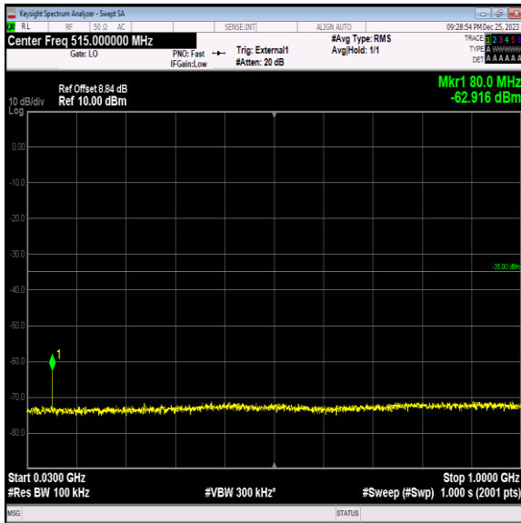
Band41_15MHz_QPSK_41165_1RB#0_30~1000_30~1000
