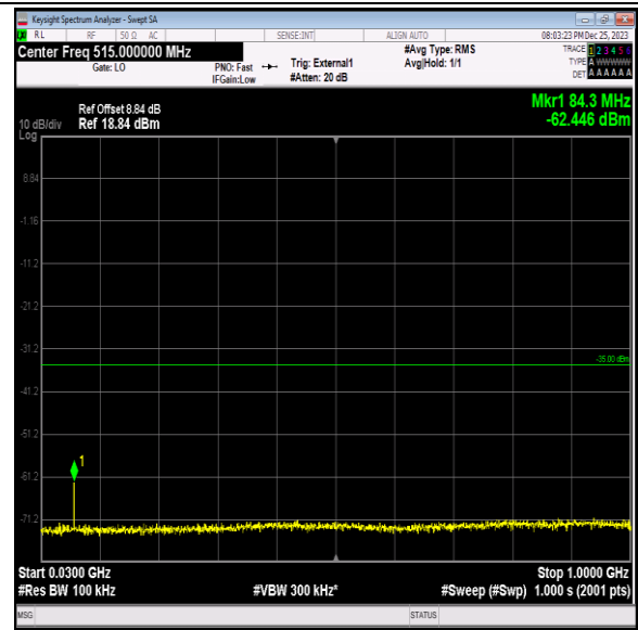
Band41_10MHz_QPSK_41190_1RB#0_30~1000_30~1000
