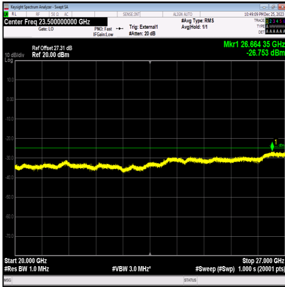
Band41_20MHz_QPSK_40640_1RB#0_20000~27000_20000~27000
