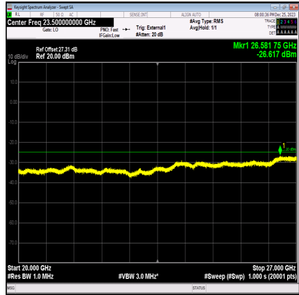
Band41_10MHz_16QAM_40640_1RB#0_20000~27000_20000~27000
