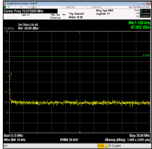
Band41_15MHz_QPSK_40115_1RB#0_0.15~30_0.15~30
