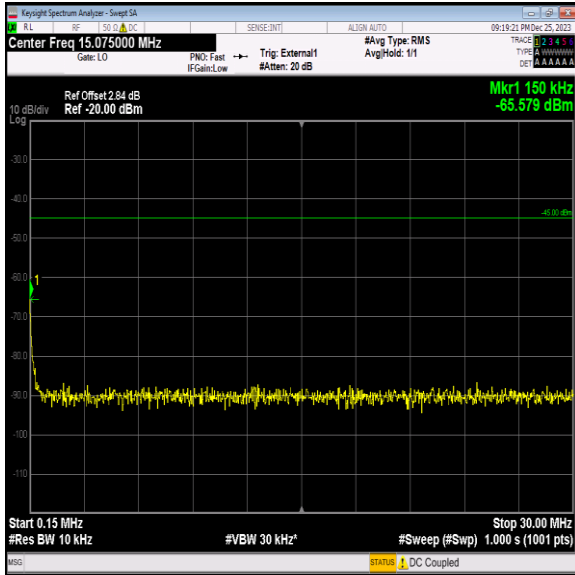
Band41_15MHz_16QAM_40115_1RB#0_0.15~30_0.15~30
