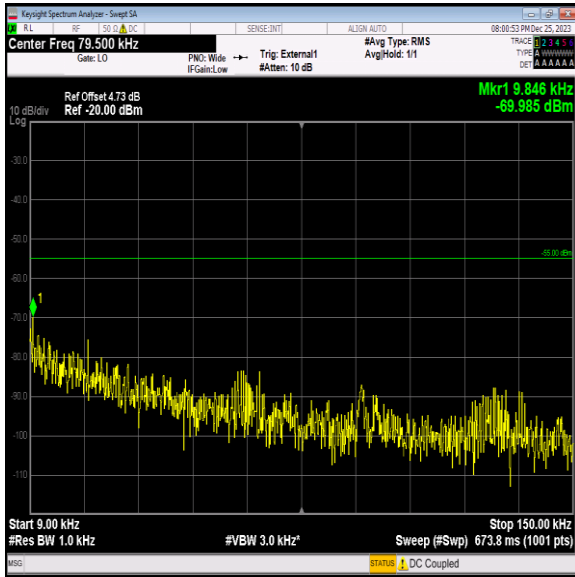
Band41_10MHz_64QAM_40640_1RB#0_0.009~0.15_0.009~0.15
