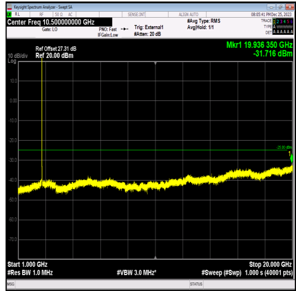
Band41_10MHz_16QAM_41190_1RB#0_1000~20000_1000~20000
