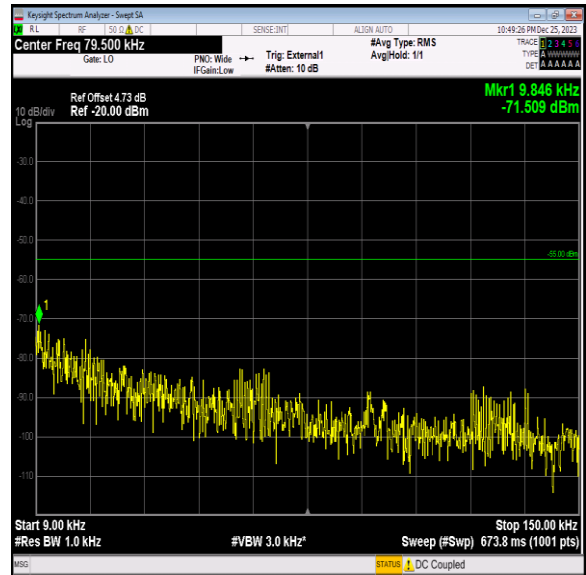
Band41_20MHz_16QAM_40640_1RB#0_0.009~0.15_0.009~0.15
