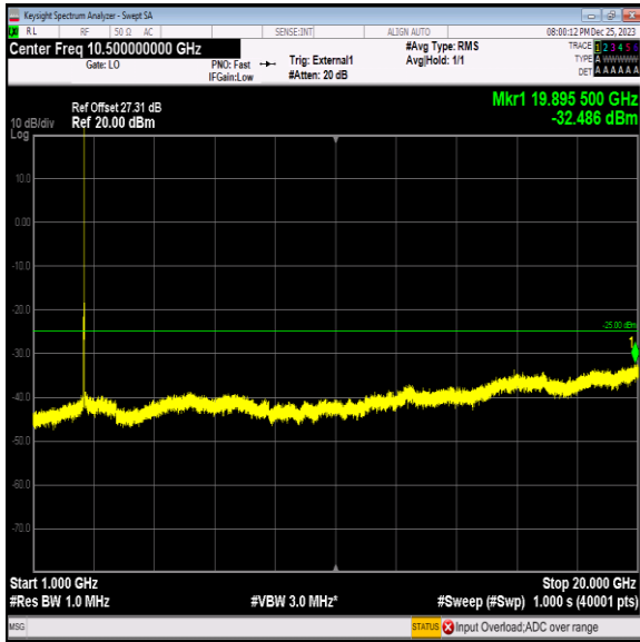
Band41_10MHz_16QAM_40640_1RB#0_1000~20000_1000~20000
