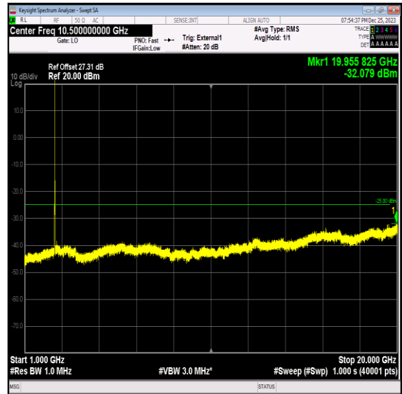
Band41_10MHz_16QAM_40090_1RB#0_1000~20000_1000~20000
