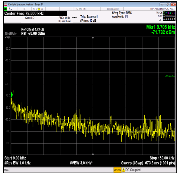
Band41_20MHz_QPSK_40140_1RB#0_0.009~0.15_0.009~0.15
