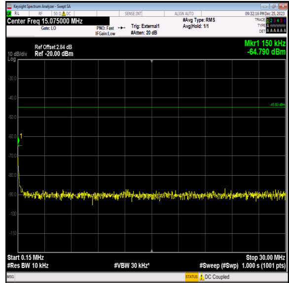
Band41_15MHz_64QAM_41165_1RB#0_0.15~30_0.15~30
