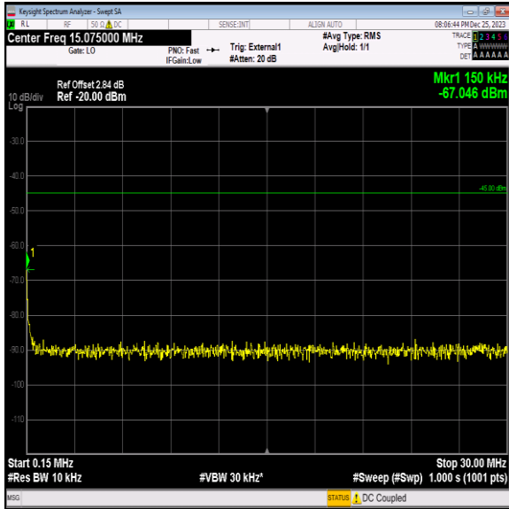
Band41_10MHz_64QAM_41190_1RB#0_0.15~30_0.15~30
