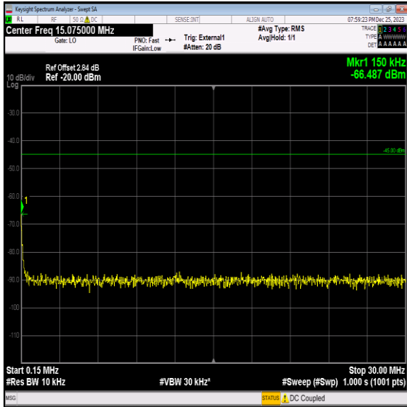
Band41_10MHz_16QAM_40640_1RB#0_0.15~30_0.15~30
