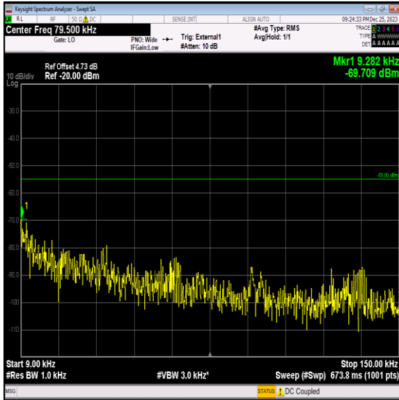
Band41_15MHz_16QAM_40640_1RB#0_0.009~0.15_0.009~0.15
