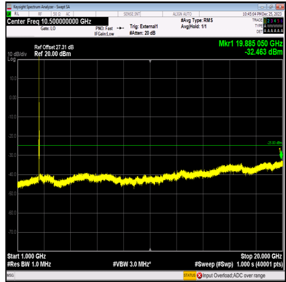
Band41_20MHz_16QAM_40140_1RB#0_1000~20000_1000~20000
