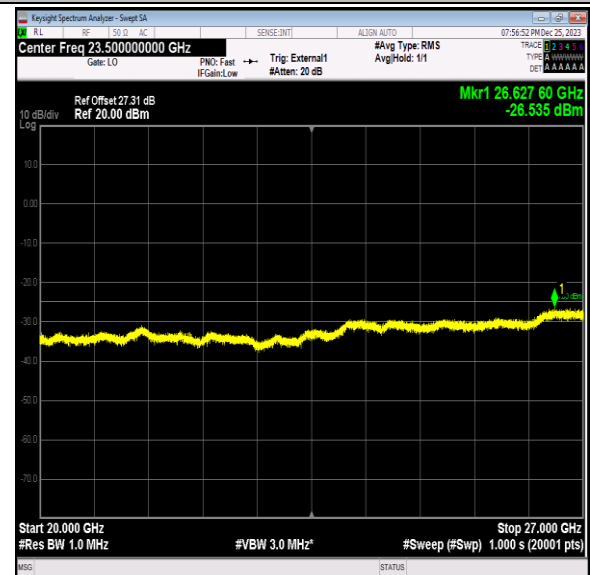
Band41_10MHz_64QAM_40090_1RB#0_20000~27000_20000~27000
