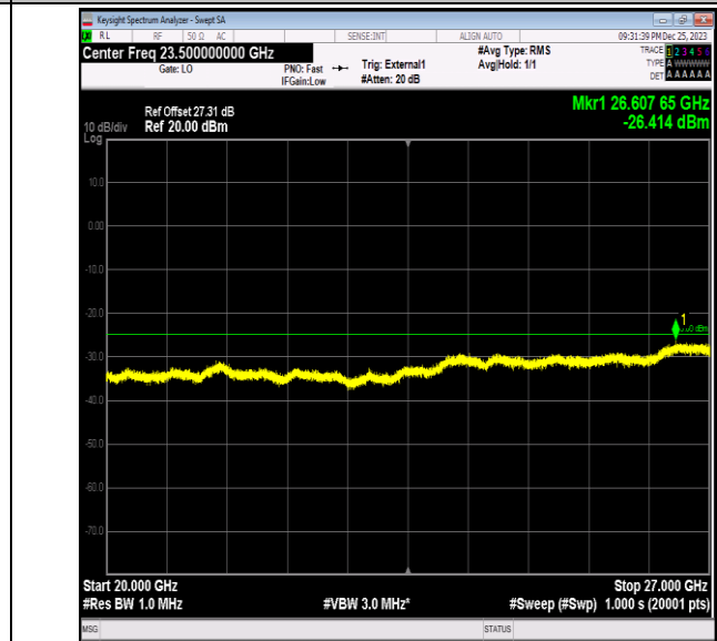
Band41_15MHz_16QAM_41165_1RB#0_20000~27000_20000~27000
