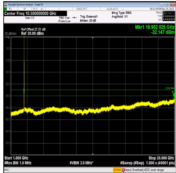
Band41_15MHz_64QAM_40115_1RB#0_1000~20000_1000~20000
