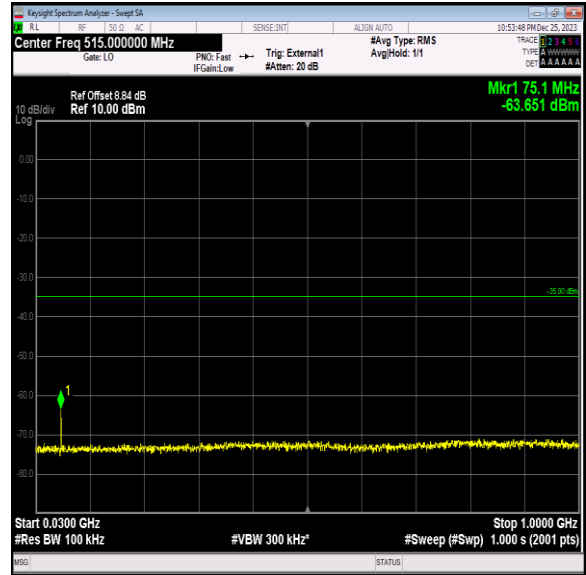
Band41_20MHz_QPSK_41140_1RB#0_30~1000_30~1000
