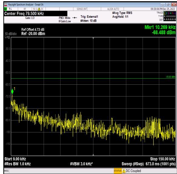
Band41_15MHz_16QAM_41165_1RB#0_0.009~0.15_0.009~0.15
