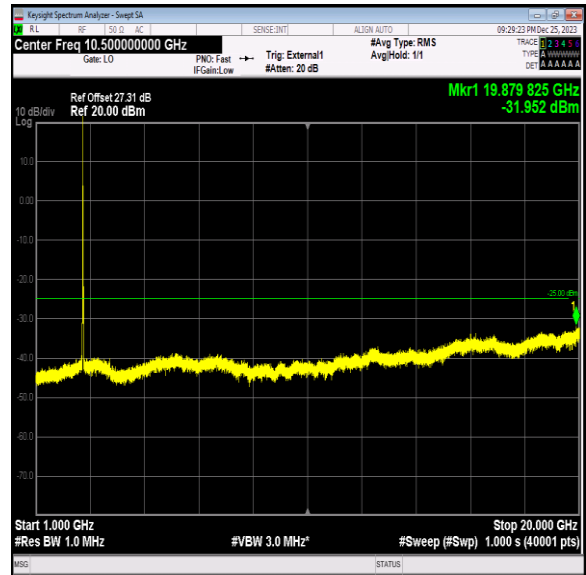
Band41_15MHz_QPSK_41165_1RB#0_1000~20000_1000~20000
