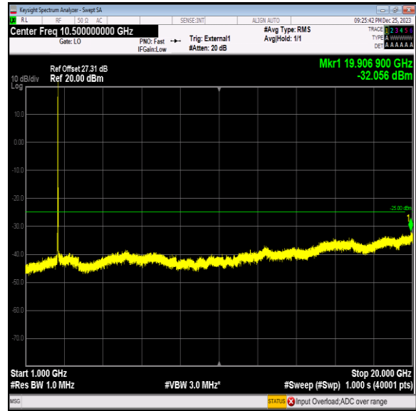
Band41_15MHz_16QAM_40640_1RB#0_1000~20000_1000~20000
