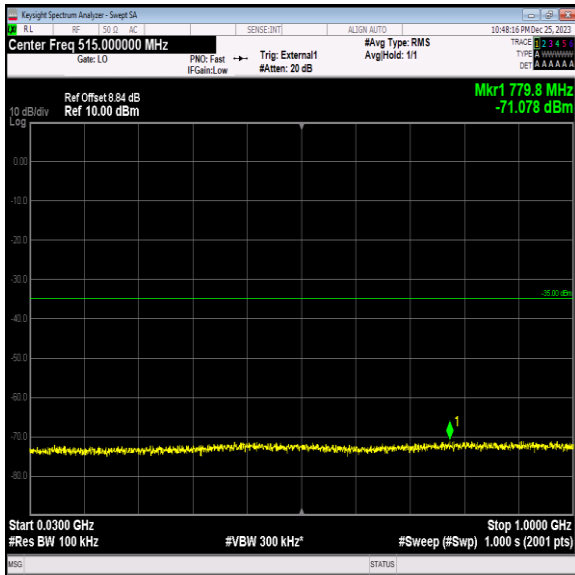
Band41_20MHz_QPSK_40640_1RB#0_30~1000_30~1000
