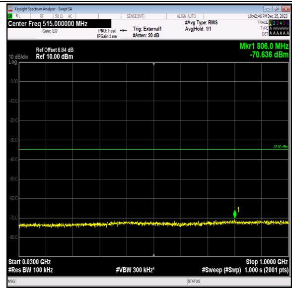
Band41_20MHz_QPSK_40140_1RB#0_30~1000_30~1000
