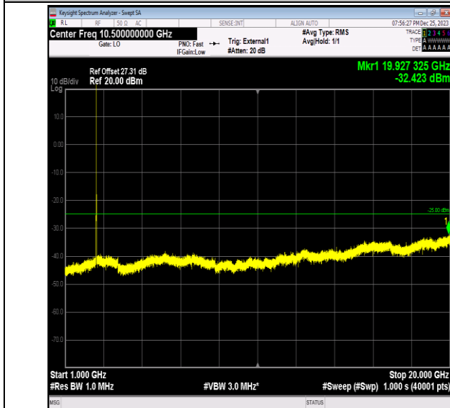
Band41_10MHz_64QAM_40090_1RB#0_1000~20000_1000~20000
