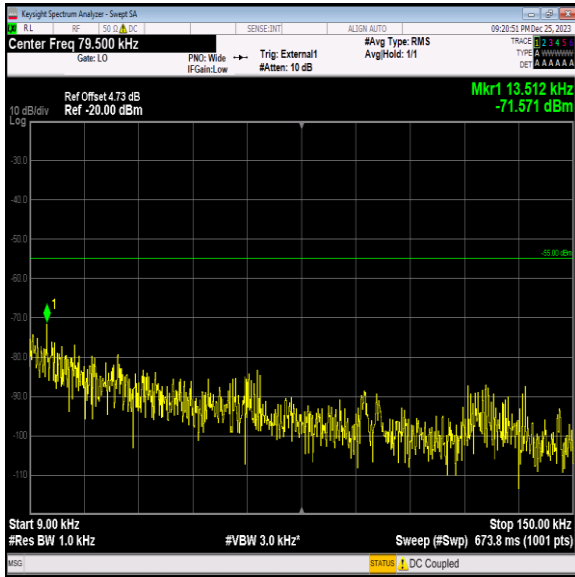
Band41_15MHz_64QAM_40115_1RB#0_0.009~0.15_0.009~0.15
