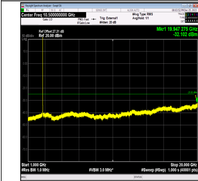
Band41_10MHz_QPSK_41190_1RB#0_1000~20000_1000~20000
