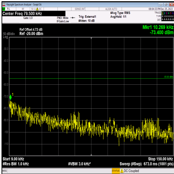
Band41_10MHz_16QAM_41190_1RB#0_0.009~0.15_0.009~0.15
