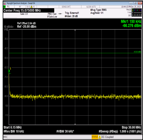
Band41_20MHz_16QAM_40140_1RB#0_0.15~30_0.15~30
