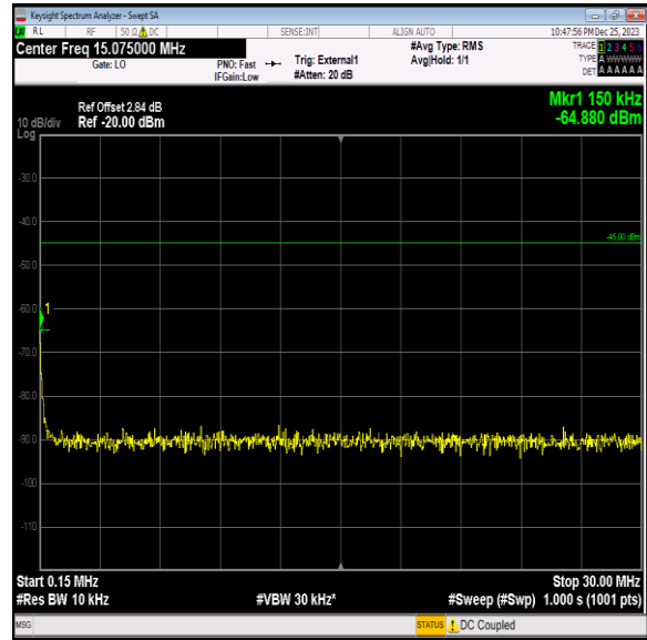
Band41_20MHz_QPSK_40640_1RB#0_0.15~30_0.15~30
