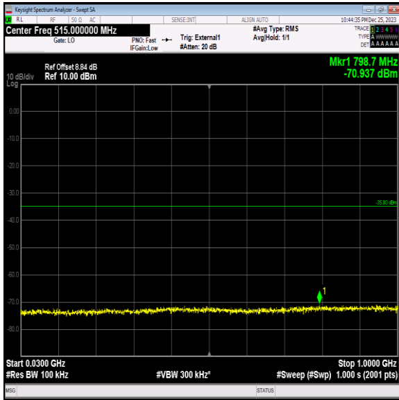
Band41_20MHz_16QAM_40140_1RB#0_30~1000_30~1000
