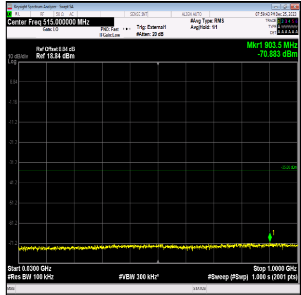
Band41_10MHz_16QAM_40640_1RB#0_30~1000_30~1000
