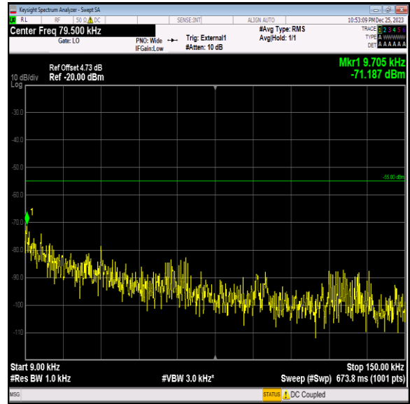
Band41_20MHz_QPSK_41140_1RB#0_0.009~0.15_0.009~0.15
