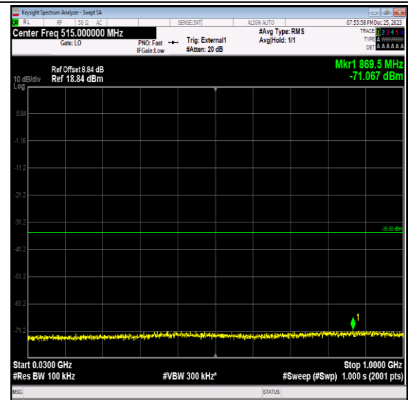
Band41_10MHz_64QAM_40090_1RB#0_30~1000_30~1000
