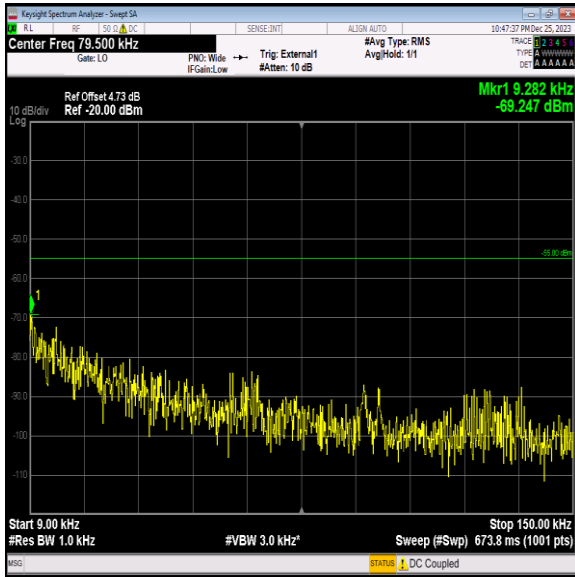
Band41_20MHz_QPSK_40640_1RB#0_0.009~0.15_0.009~0.
