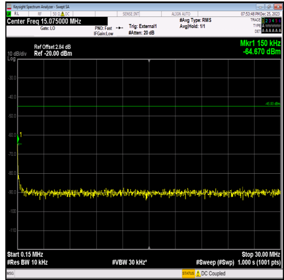
Band41_10MHz_16QAM_40090_1RB#0_0.15~30_0.15~30
