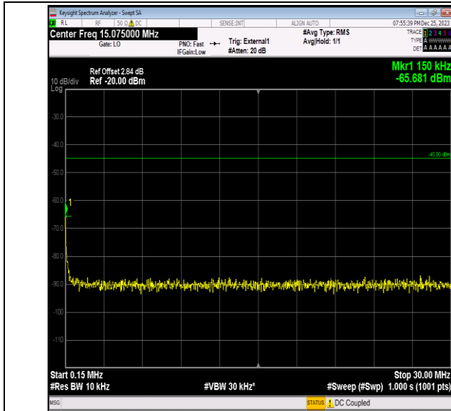
Band41_10MHz_64QAM_40090_1RB#0_0.15~30_0.15~30
