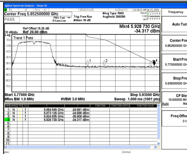
11N40MIMO-Ant2-5795-PASS
