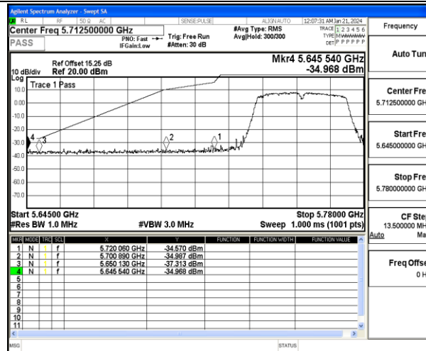
11N40MIMO-Ant2-5755-PASS
