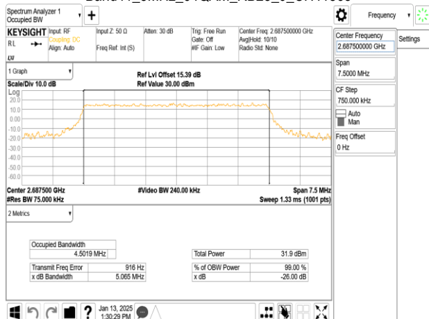
Band41_5MHz_256QAM_RB25_0_CH41565
