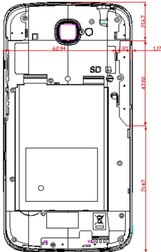
b2.Diversity Antenna
