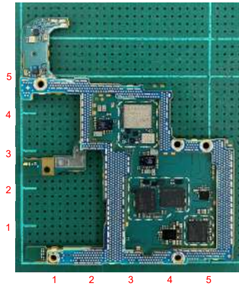
Internal Main-PWB Rear without Shield case (Front-side)
