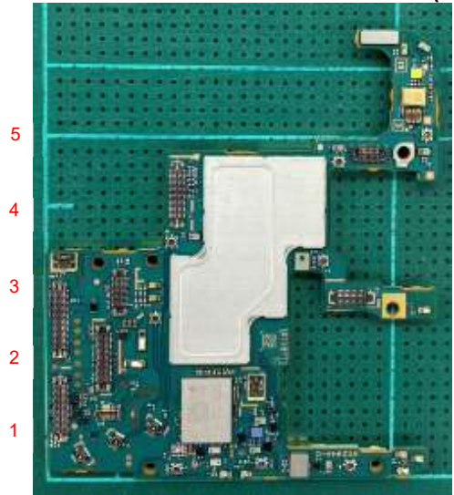
Internal Main-PWB Rear with Shield case (Rear-side)
