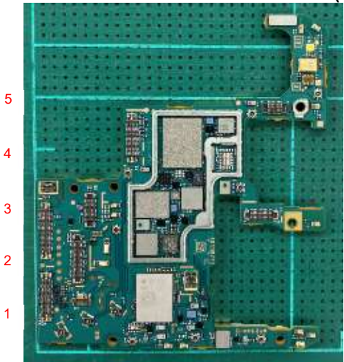
Internal Main-PWB Rear with Shield case (Front-side)
