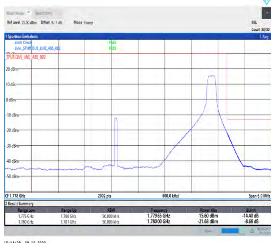
1-N66-PC3-15-5-H-5-CP-QPSK-Edge_1RB_Right-1@ 24-Ant1-1-seegraph-PASS-see graph
