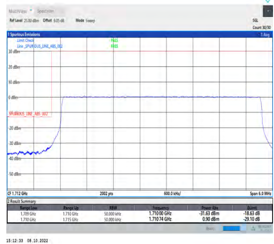
1-N66-PC3-15-5-L-6-CP-QPSK-Outer_Full-25@0 Ant1-1-seegraph-PASS-see graph
