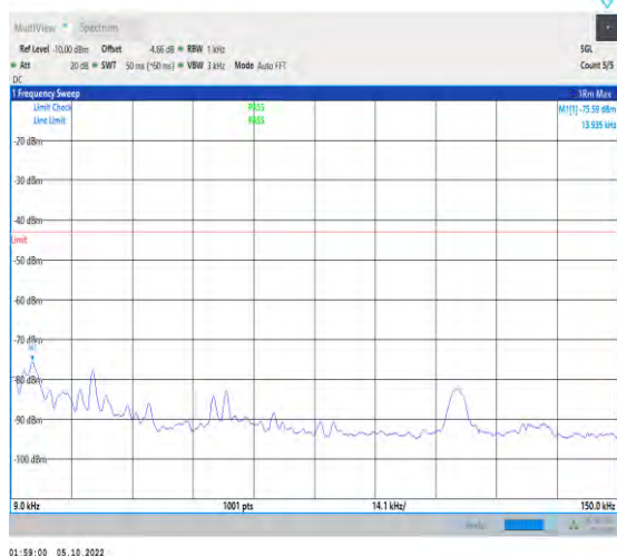
1-N66-PC3-15-40-L-1-DFT-QPSK-Inner_1RB_Left-1 @1-0.009-0.15-Ant1-0.01--75.59--43-PASS
