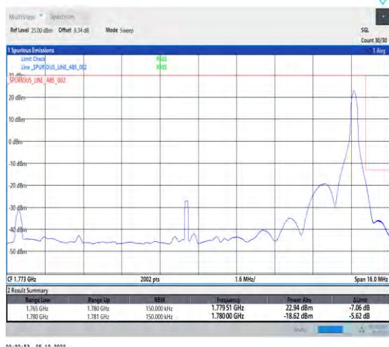
1-N66-PC3-15-15-H-2-DFT-QPSK-Edge_1RB_Right-1 @78-Ant1-1-seegraph-PASS-see graph
