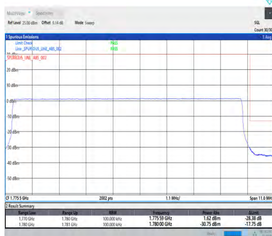
1-N66-PC3-15-10-H-6-CP-QPSK-Outer_Full-52@ 0-Ant1-1-seegraph-PASS-see graph
