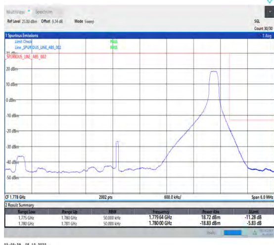
1-N66-PC3-15-5-H-2-DFT-QPSK-Edge_1RB_Right-1 @24-Ant1-1-seegraph-PASS-see graph
