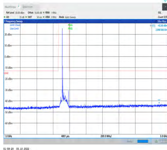
1-N66-PC3-15-40-L-1-DFT-QPSK-Inner_1RB_Left-1 @1-1000-3000-Ant1-2890.50--42.60--13-PASS
