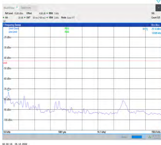
1-N66-PC3-15-40-M-1-DFT-QPSK-Inner_1RB_Left-1 @1-0.009-0.15-Ant1-0.01--75.14--43-PASS
