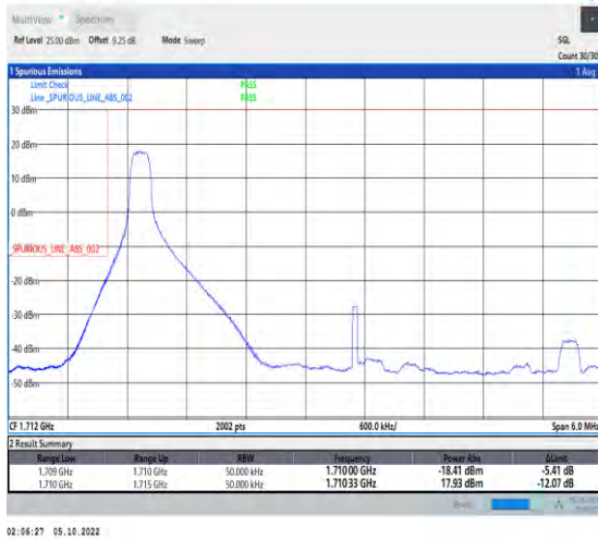
1-N66-PC3-15-5-L-1-DFT-QPSK-Edge_1RB_Left-1@0 -Ant1-1-seegraph-PASS-see graph
