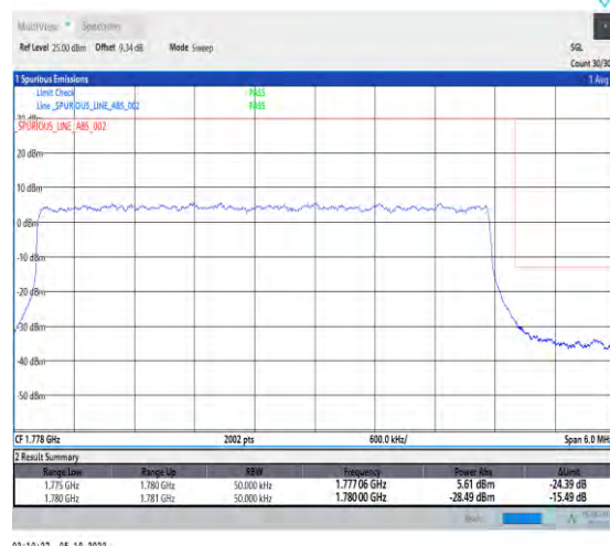
1-N66-PC3-15-5-H-3-DFT-QPSK-Outer_Full-25@ 0-Ant1-1-seegraph-PASS-see graph
