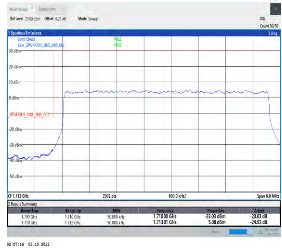
1-N66-PC3-15-5-L-3-DFT-QPSK-Outer_Full-25@0 -Ant1-1-seegraph-PASS-see graph
