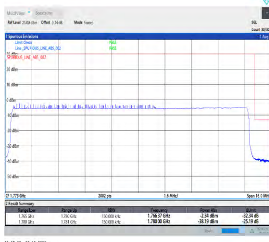
1-N66-PC3-15-15-H-6-CP-QPSK-Outer_Full-79@ 0-Ant1-1-seegraph-PASS-see graph
