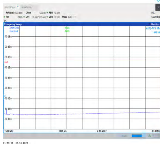
1-N66-PC3-15-40-L-1-DFT-QPSK-Inner_1RB_Left-1 @1-0.15-30-Ant1-0.15--71.19--33-PASS
