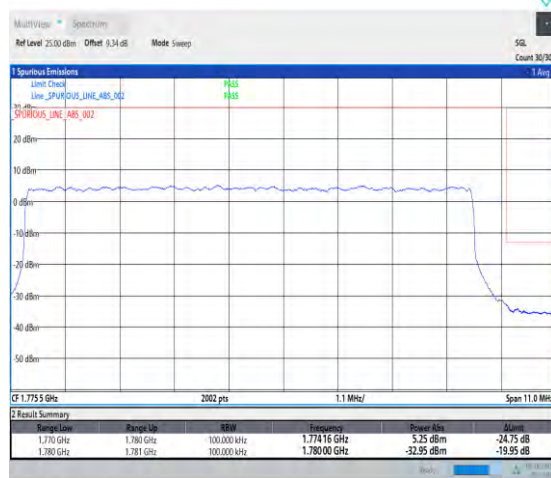
1-N66-PC3-15-10-H-3-DFT-QPSK-Outer_Full-50 @0-Ant1-1-seegraph-PASS-see graph
