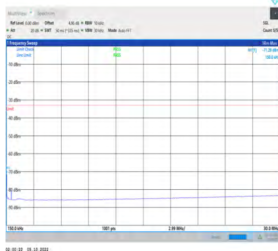
1-N66-PC3-15-40-M-1-DFT-QPSK-Inner_1RB_Left-1 @1-0.15-30-Ant1-0.15--71.29--33-PASS
