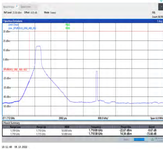
1-N66-PC3-15-5-L-4-CP-QPSK-Edge_1RB_Left-1@0 Ant1-1-seegraph-PASS-see graph
