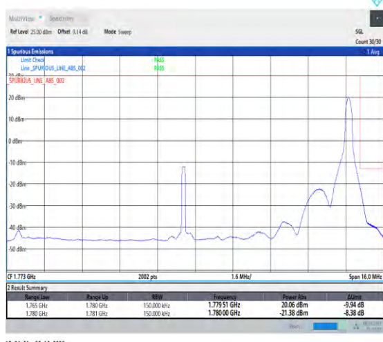
1-N66-PC3-15-15-H-5-CP-QPSK-Edge_1RB_Right-1 @78-Ant1-1-seegraph-PASS-see graph
