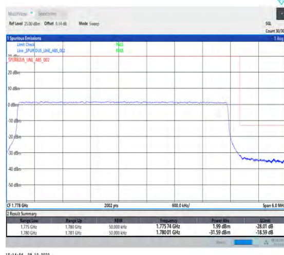
1-N66-PC3-15-5-H-6-CP-QPSK-Outer_Full-25@0- Ant1-1-seegraph-PASS-see graph
