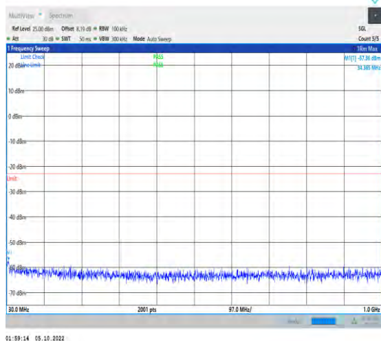
1-N66-PC3-15-40-L-1-DFT-QPSK-Inner_1RB_Left-1 @1-30-1000-Ant1-34.37--57.36--23-PASS
