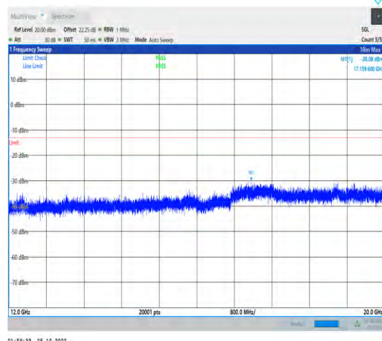
1-N66-PC3-15-40-L-1-DFT-QPSK-Inner_1RB_Left-1 @1-12000-20000-Ant1-17159.60--30.08--13-PASS
