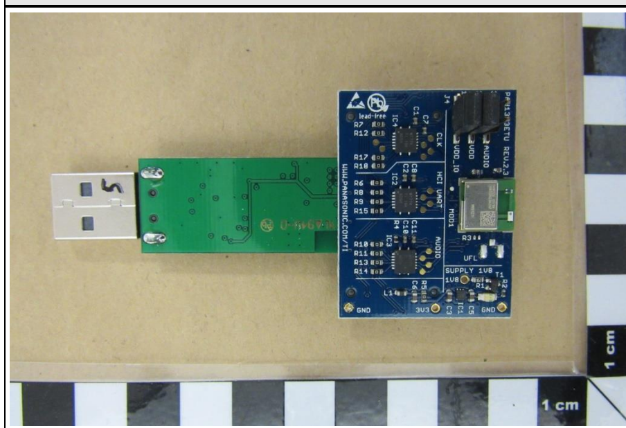
Evaluation Board with Module ENW89823A5KF, Top View
