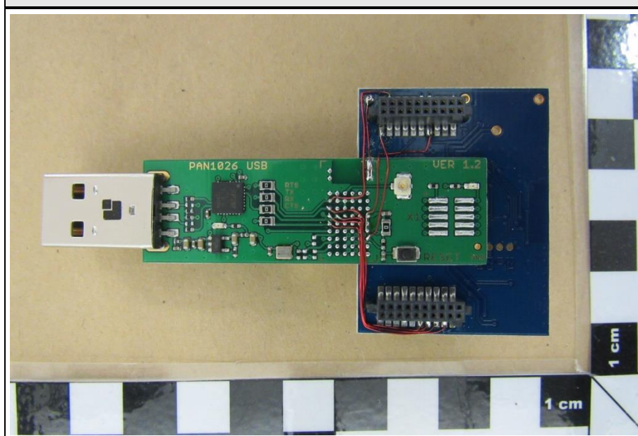
Evaluation Board with Module ENW89823A5KF, Bottom View
