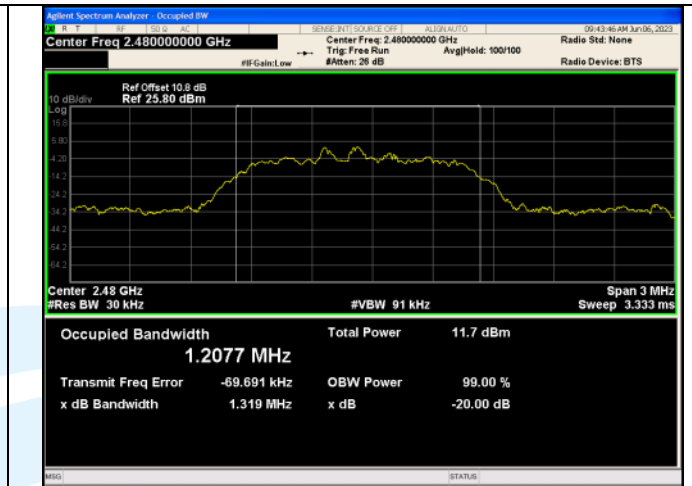
\pi/4 DQPSK_2-DH5_Channel 78
