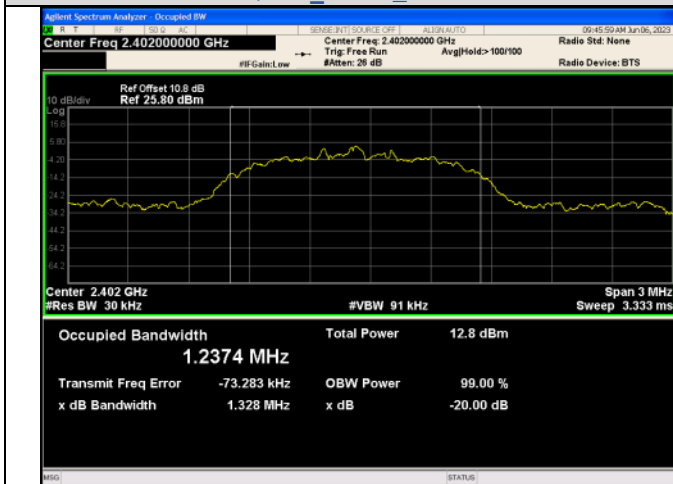
8DPSK_3-DH5_Channel 0
