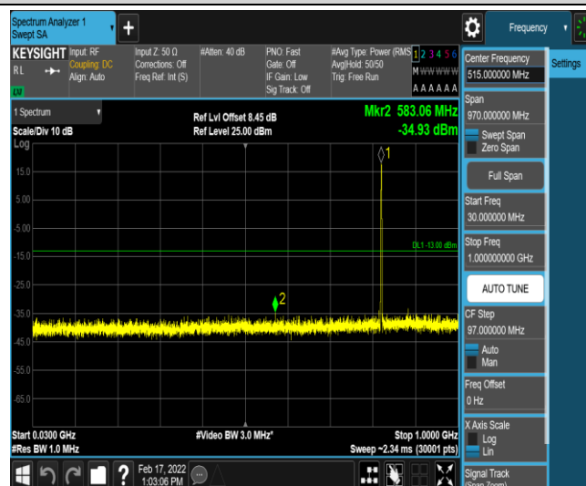
Band26-10MHz-16QAM-26840-1-0-Low-30-1000--34.93-PASS
