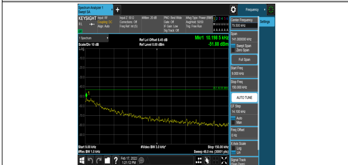
Band26-15MHz-QPSK-26865-1-0-Low-0.009-0.15--51.88-PASS
