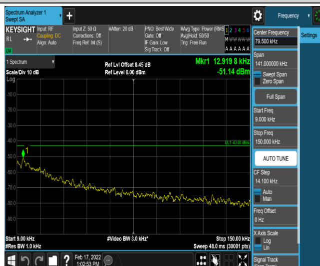
Band26-10MHz-16QAM-26840-1-0-Low-0.009-0.15--51.15-PASS
