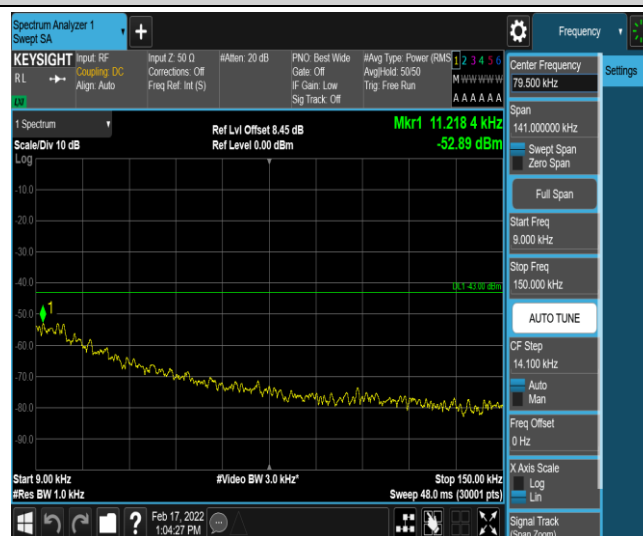
Band26-10MHz-QPSK-26915-1-0-Low-0.009-0.15--52.89-PASS
