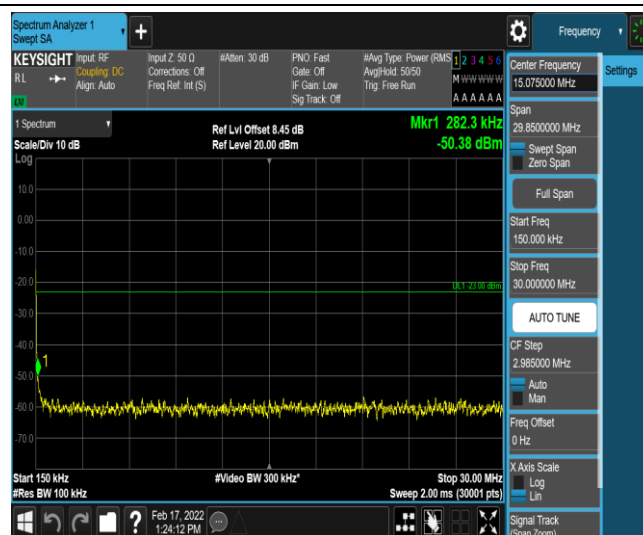
Band26-15MHz-QPSK-26915-1-0-Low-0.15-30--50.38-PASS
