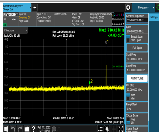
Band26-15MHz-QPSK-26965-1-0-High-30-1000--34.83-PASS
