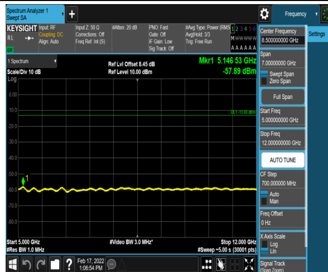
Band26-10MHz-16QAM-26915-1-0-Low-5000-12000--57.89-PASS
