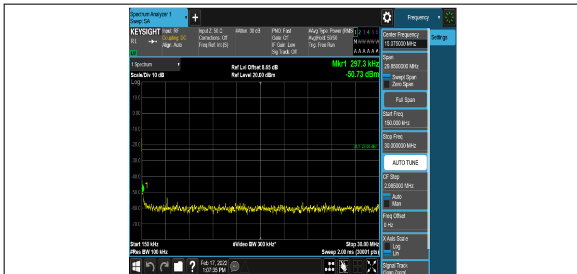
Band26-10MHz-QPSK-26990-1-0-High-0.15-30--50.73-PASS
