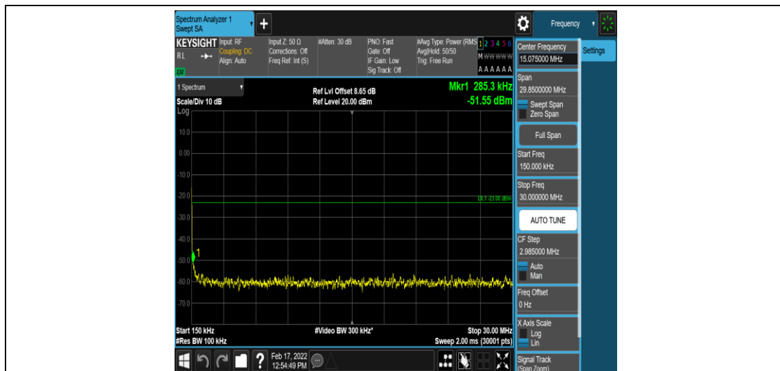
Band26-5MHz-16QAM-27015-1-0-High-0.15-30--51.55-PASS
