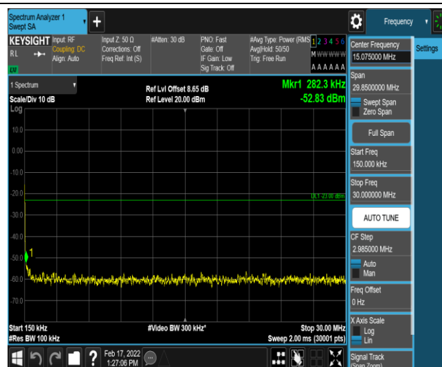
Band26-15MHz-QPSK-26965-1-0-High-0.15-30--52.83-PASS
