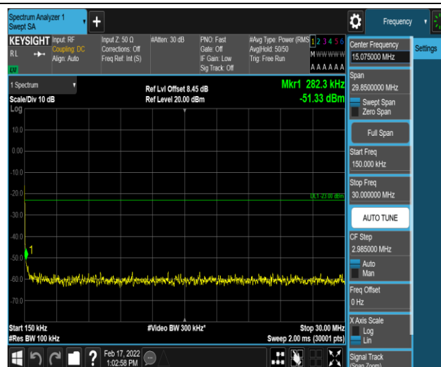
Band26-10MHz-16QAM-26840-1-0-Low-0.15-30--51.33-PASS
