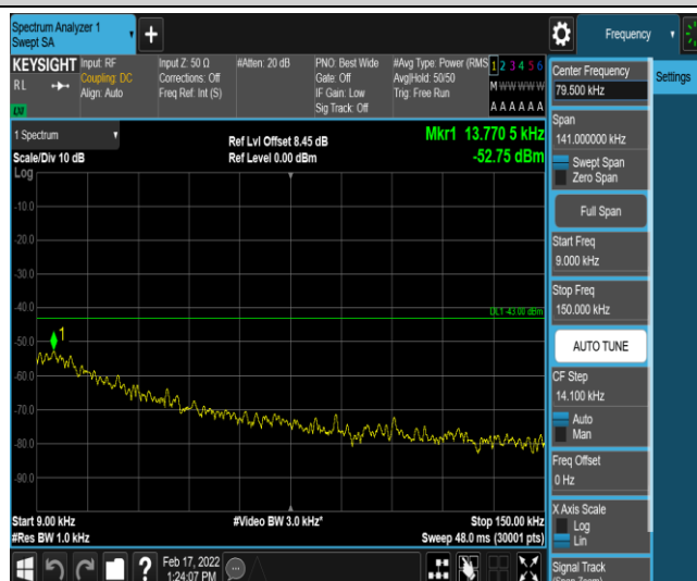
Band26-15MHz-QPSK-26915-1-0-Low-0.009-0.15--52.75-PASS
