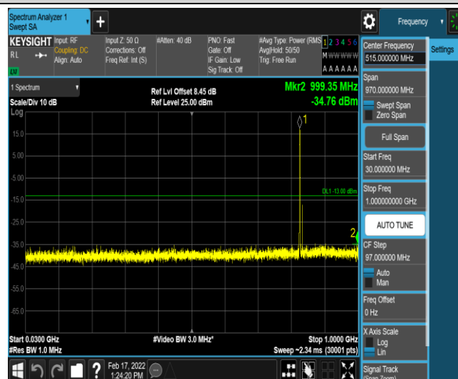
Band26-15MHz-QPSK-26915-1-0-Low-30-1000--34.76-PASS
