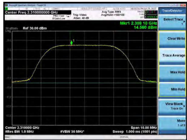
LTE Band 30 64QAM 10MHz
