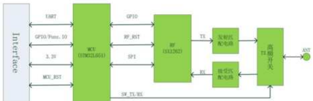
Figure 2-2 Hardware system block diagram
