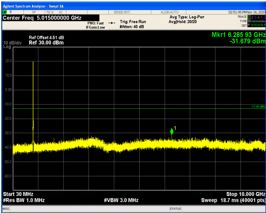
LTE Band5 QPSK BW=10MHz Channel=20450 RB Size=1 Position=#0
