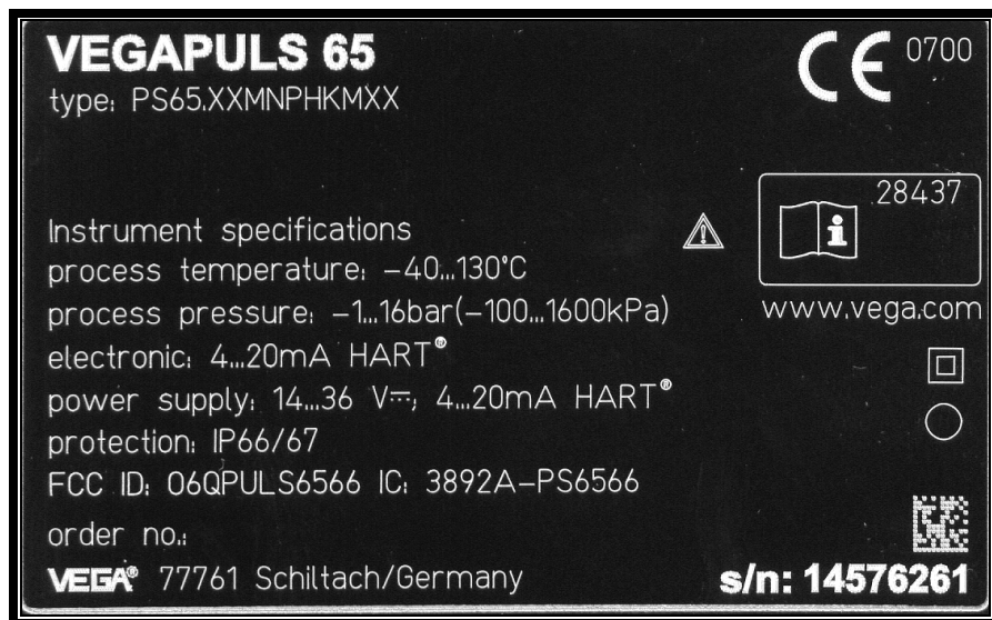
Photograph 1: FCC ID & IC ID Label Sample – VEGAPULS 65
