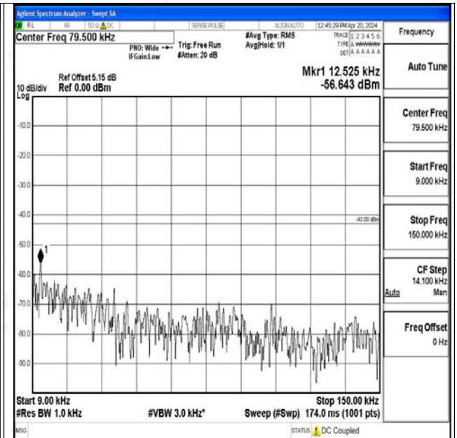
Band25_15MHz_16QAM_26115_1RB#0_0.009~0.15_0.009~0.15
