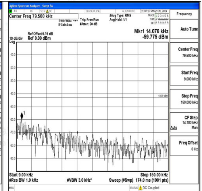
Band25_20MHz_16QAM_26365_1RB#0_0.009~0.15_0. 009~0.15
