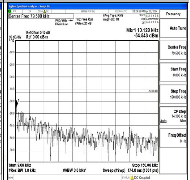
Band25_20MHz_16QAM_26590_1RB#0_0.009~0.15_0.009~0.15
