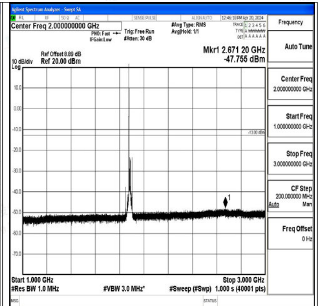
Band25_15MHz_QPSK_26365_1RB#0_1000~3000_1000~3000
