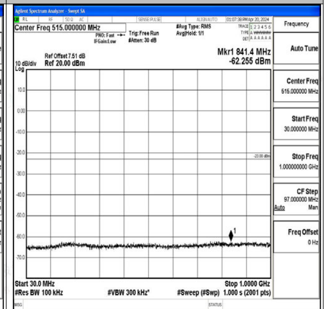
Band25_20MHz_16QAM_26365_1RB#0_30~1000_30~1 000
