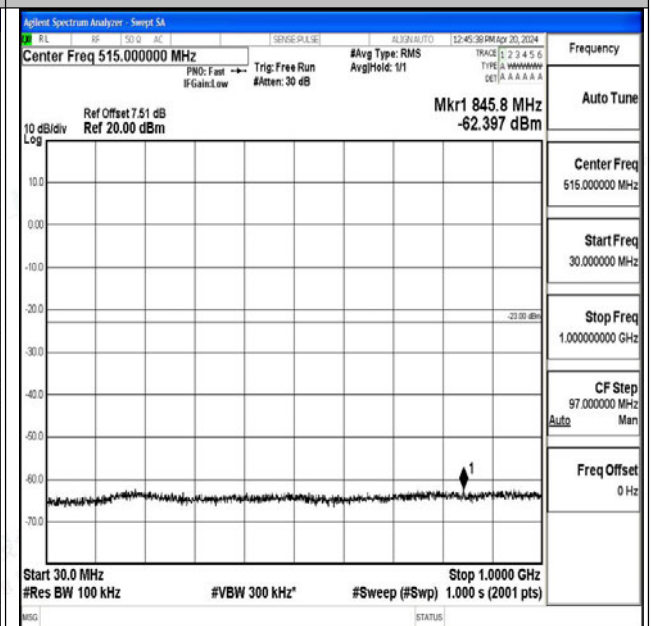
Band25_15MHz_16QAM_26115_1RB#0_30~1000_30~1000
