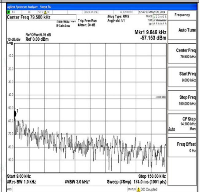
Band25_15MHz_16QAM_26365_1RB#0_0.009~0.15_0.009~0.15
