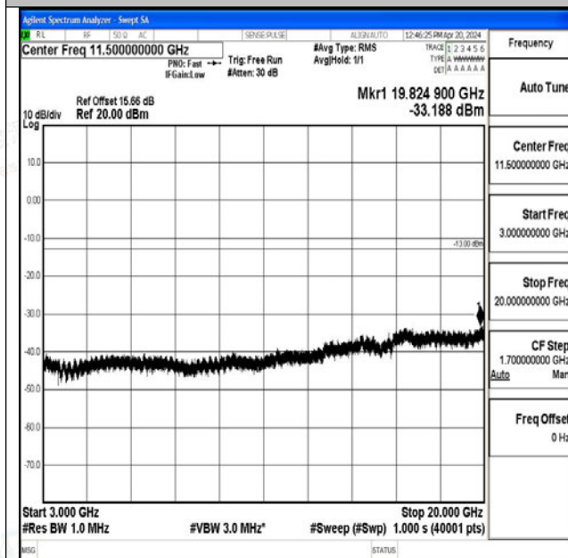
Band25_15MHz_QPSK_26365_1RB#0_3000~20000_3000~20000
