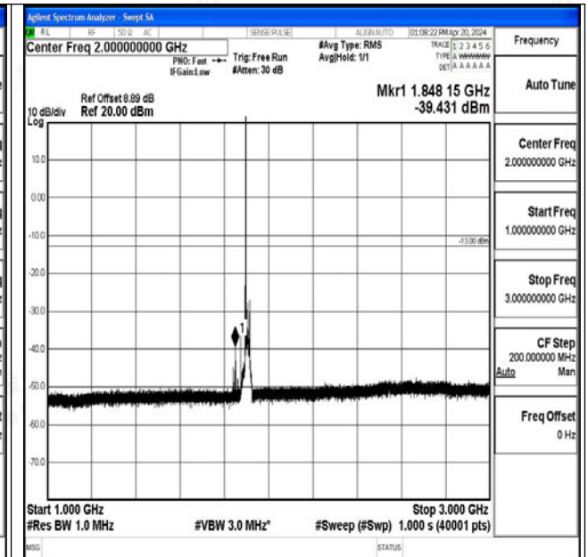
Band25_20MHz_QPSK_26590_1RB#0_1000~3000_1000~3000
