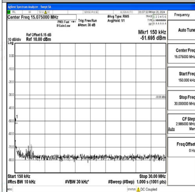
Band25_20MHz_16QAM_26365_1RB#0_0.15~30_0.15~ 30
