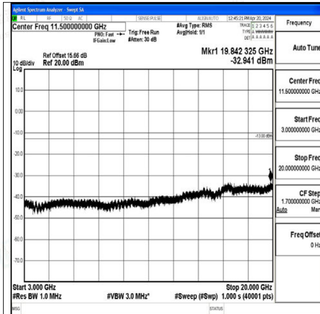
Band25_15MHz_QPSK_26115_1RB#0_3000~20000_3000~20000
