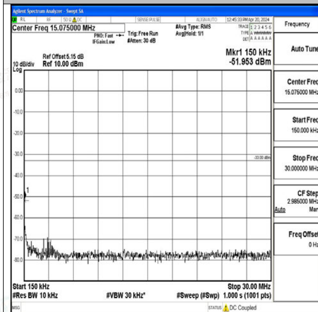
Band25_15MHz_16QAM_26115_1RB#0_0.15~30_0.15~30
