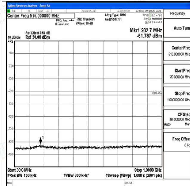
Band25_15MHz_QPSK_26365_1RB#0_30~1000_30~1000
