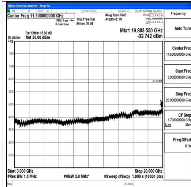
Band25_20MHz_QPSK_26365_1RB#0_3000~20000_30 00~20000
