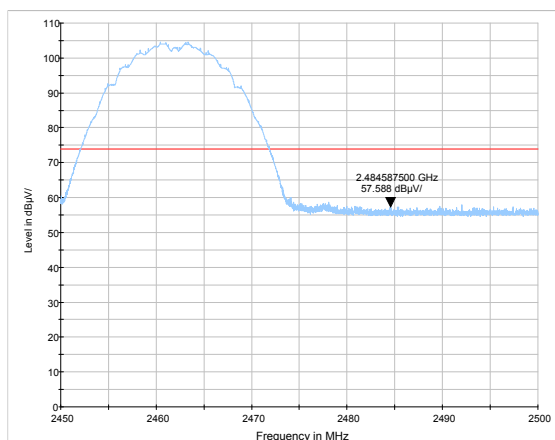
802.11b-Channel 11: Average
