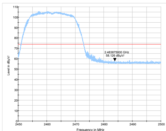
802.11g-Channel 11: Peak
