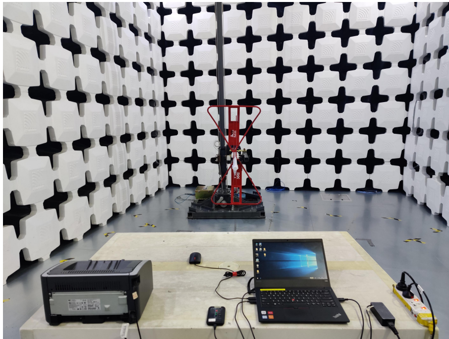
1. Radiated Emissions (Part 15B, USB mode) (30MHz- 1GHz)
