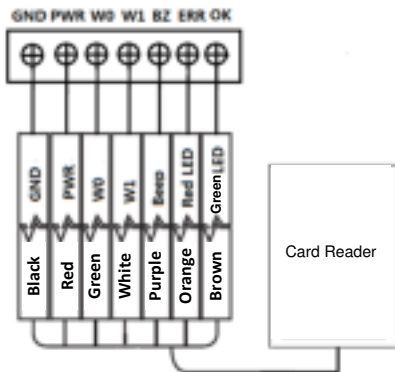
Figure 3-4 Wiring for Wiegand Communication Mode
