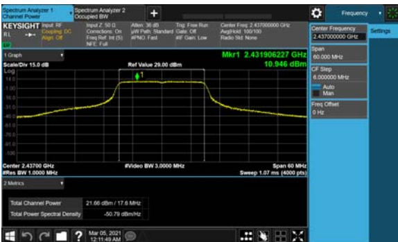
Antenna C
