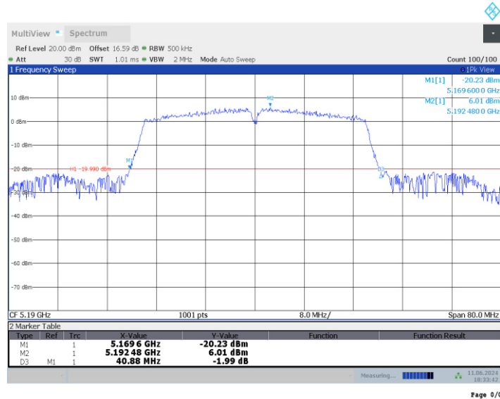
Fig.21 26dB Emission Bandwidth (802.11n-HT40, 5190MHz)
