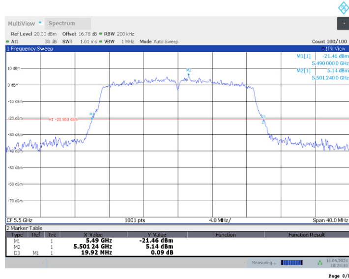
Fig.17 26dB Emission Bandwidth (802. 11n-HT20, 5500MHz)
