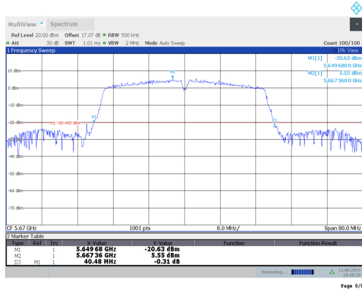
Fig.27 26dB Emission Bandwidth (802. 11n-HT40, 5670MHz)
