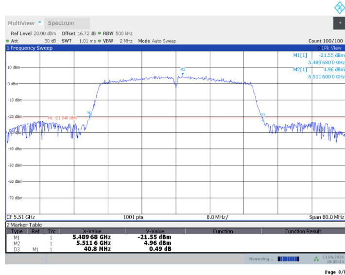
Fig.25 26dB Emission Bandwidth (802. 11n-HT40, 5510MHz)
