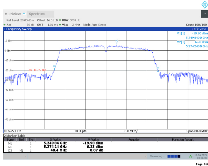
Fig.23 26dB Emission Bandwidth (802.11n-HT40, 5270MHz)
