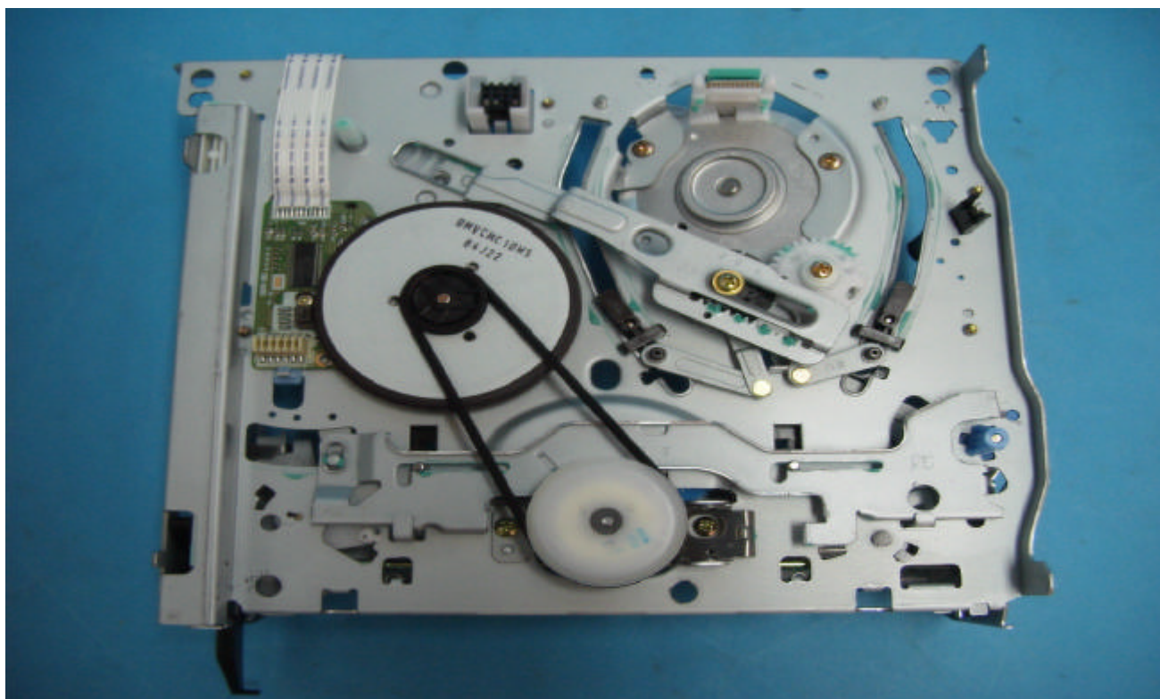
VCR Deck Bottom View
