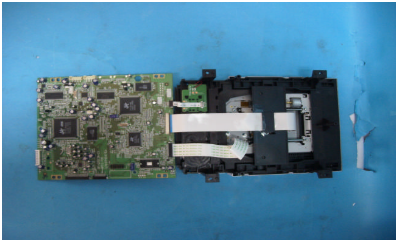
DVD Deck Top View
