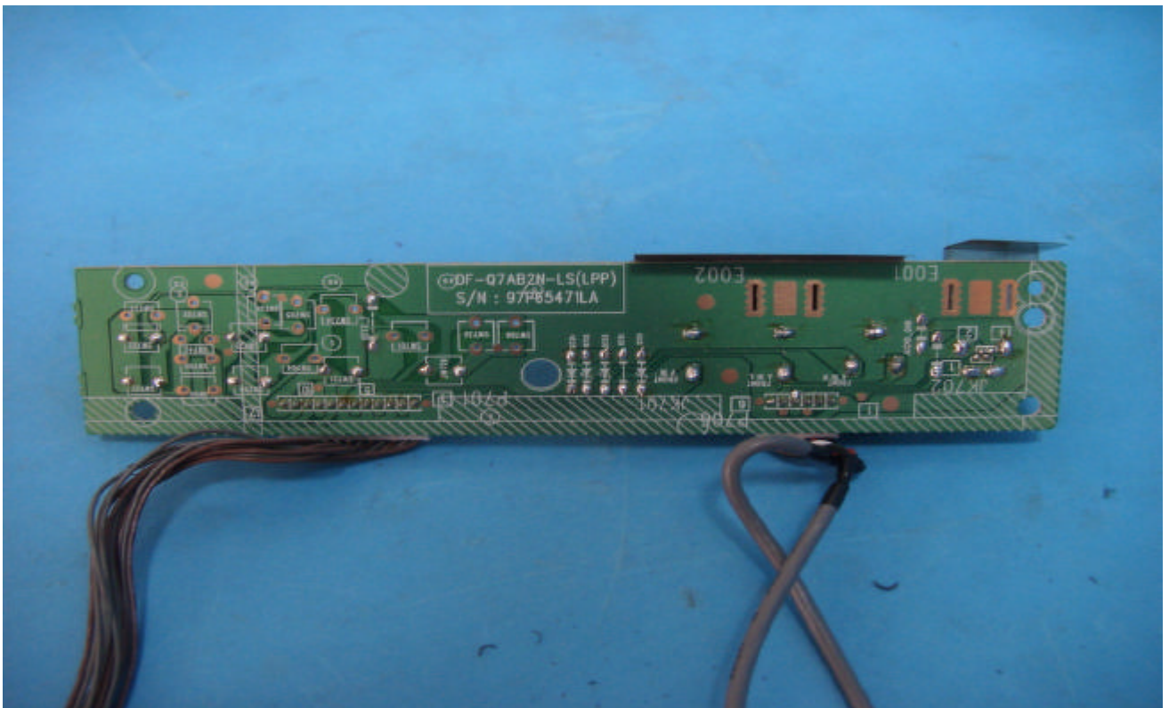
AUX front Input Panel PCB Copper View
