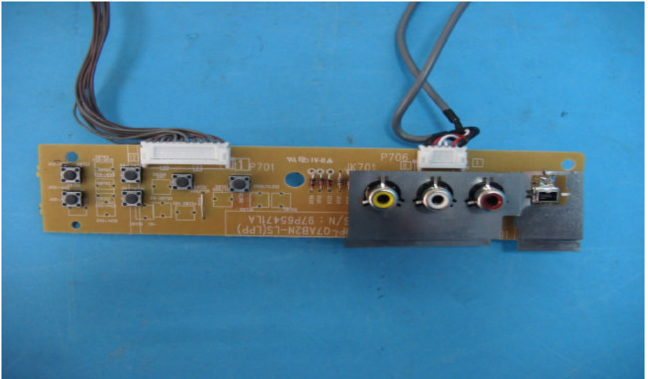
AUX front Input Panel PCB Parts View
