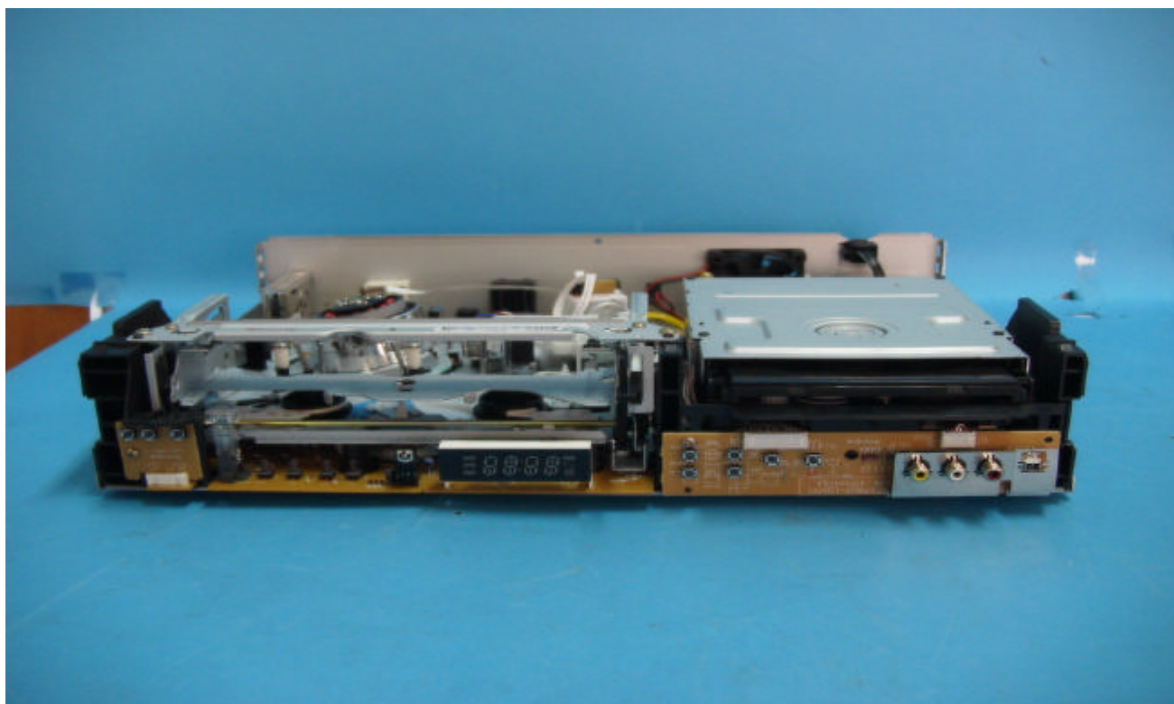
Inner Top View
