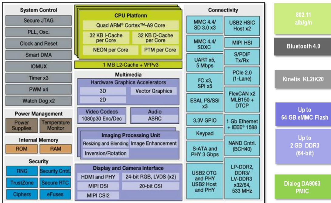
Block diagram of ConnectCore 6
