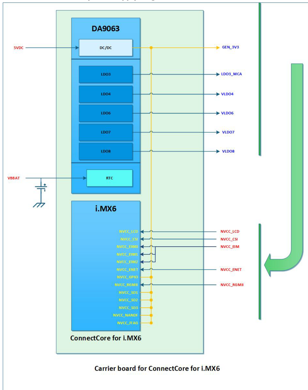
ConnectCore 6 power supply diagram
