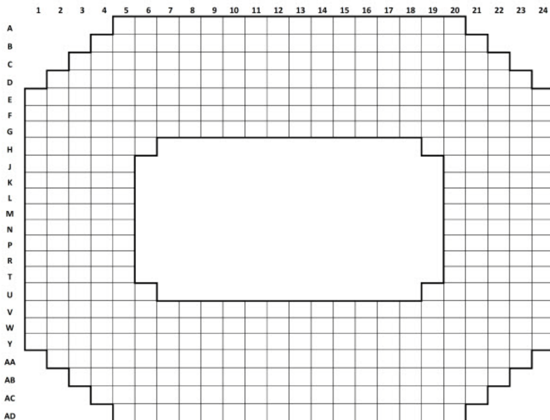
ConnectCore top view module pinout
