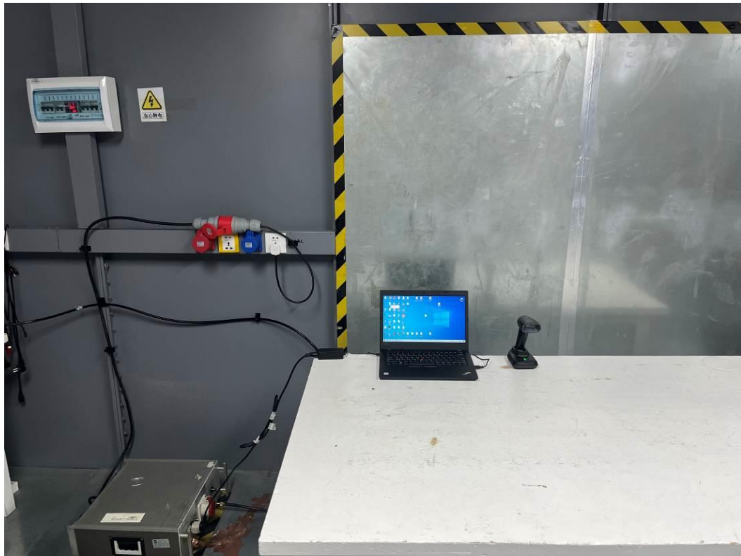
Photos of Power Line Conducted Emission Test
