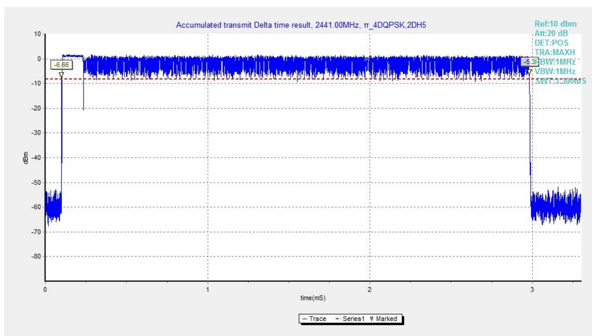
Fig. 80 Time of Occupancy (Dwell Time) ( \pi/4 DQPSK, Ch39)
