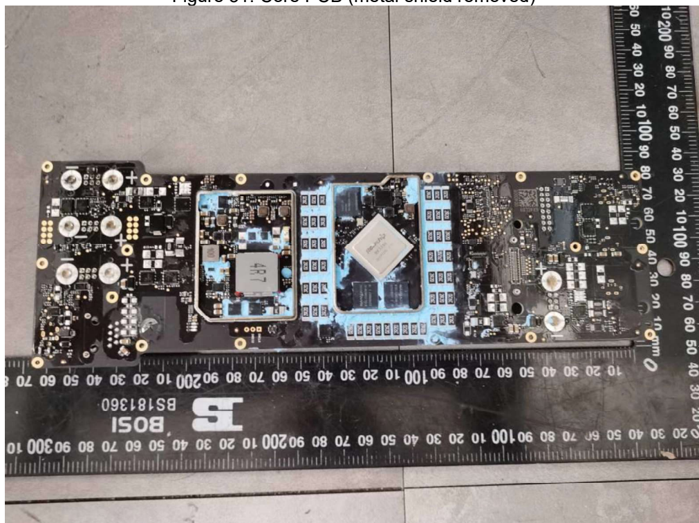
Figure 32. Core PCB (metal shield removed)
