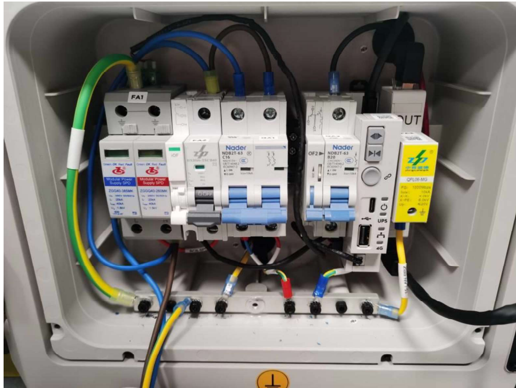
Figure 11. Internal view
