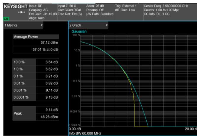
Channel: BOTTOM, Modulation: 64QAM, BW=60MHz, CCDF
