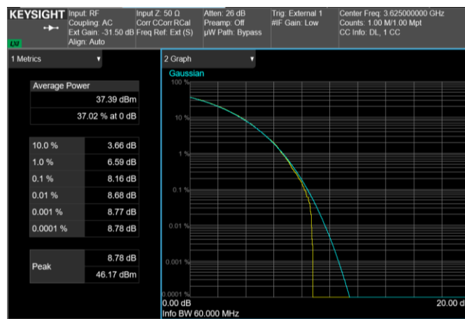
Channel: MIDDLE, Modulation: 64QAM, BW=60MHz, CCDF
