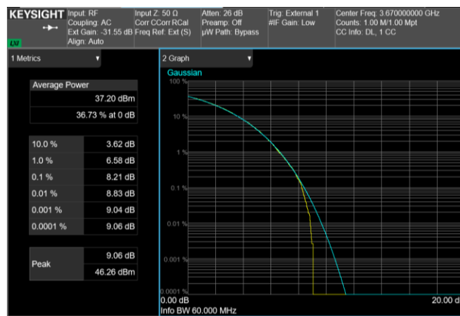
Channel: TOP, Modulation: 64QAM, BW=60MHz, CCDF
