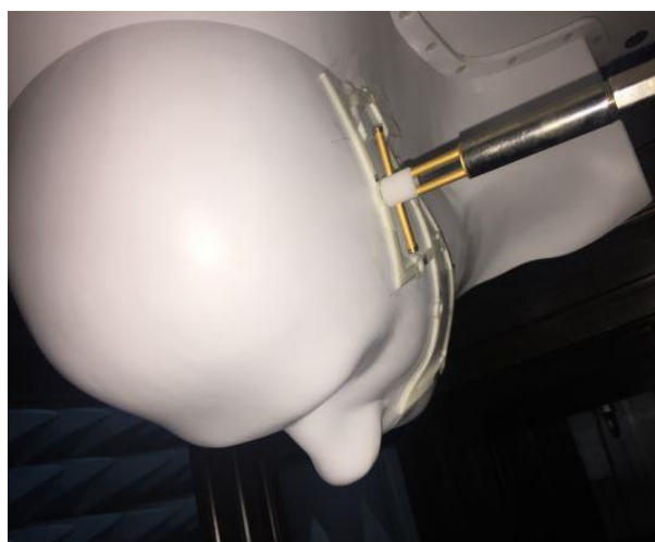
Setup Photo at SAM Face-Down Phantom
