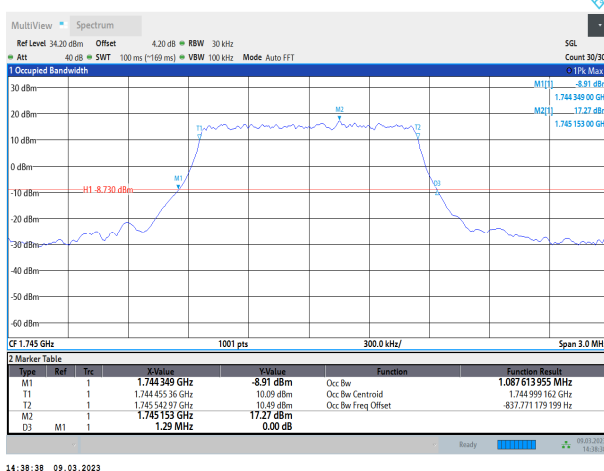
Band66-1.4MHz-QPSK-132322-6RB#0
