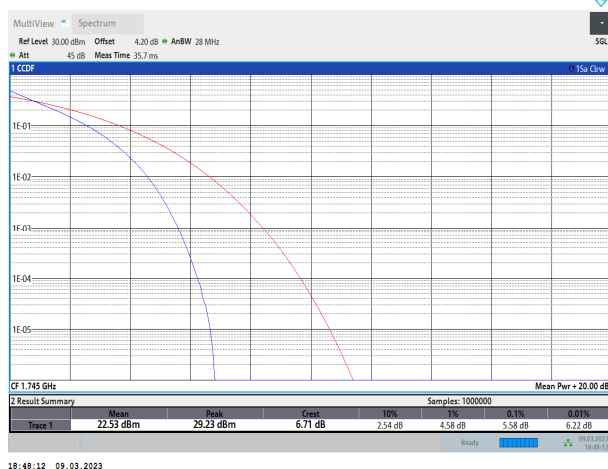
Band66-20MHz-QPSK-132322-100RB#0
