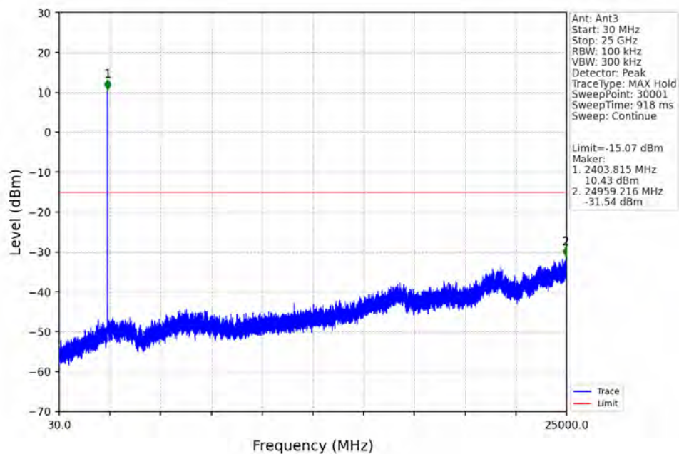
1.4M_LCH_2403.5MHz_Ant3_NTNV
