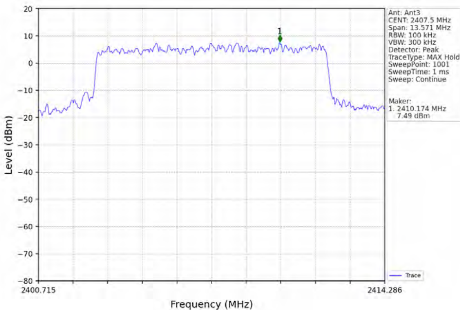
10M_LCH_2407.5MHz_Ant3_NTNV
