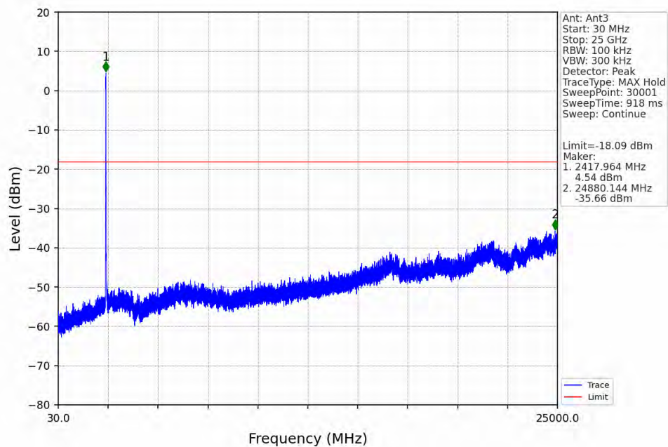
20M_LCH_2412.5MHz_Ant3_NTNV
