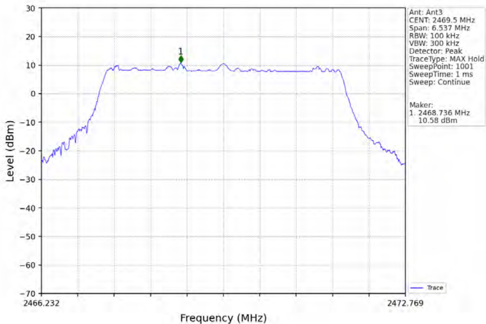
5M_HCH_2469.5MHz_Ant3_NTNV
