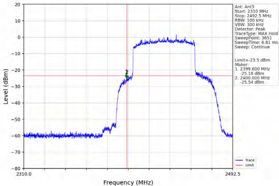
60M_LCH_2432.5MHz_Ant3_NTNV
