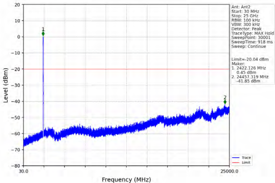
40M_LCH_2422.5MHz_Ant2_NTNV
