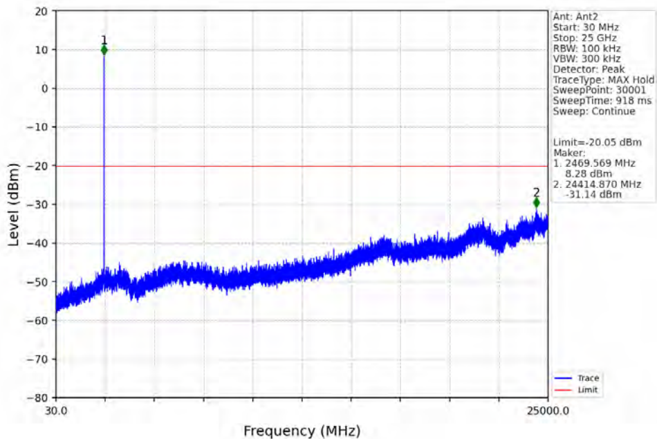
5M_HCH_2469.5MHz_Ant2_NTNV
