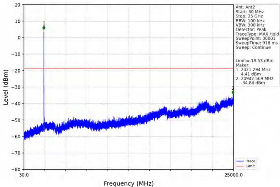
20M_LCH_2412.5MHz_Ant2_NTNV
