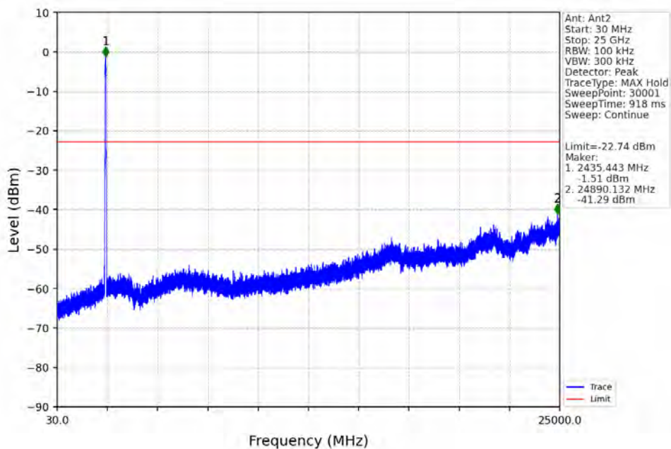
60M_LCH_2432.5MHz_Ant2_NTNV
