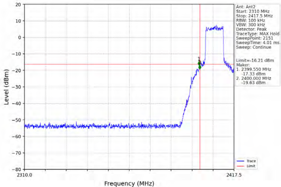
10M_LCH_2407.5MHz_Ant2_NTNV
