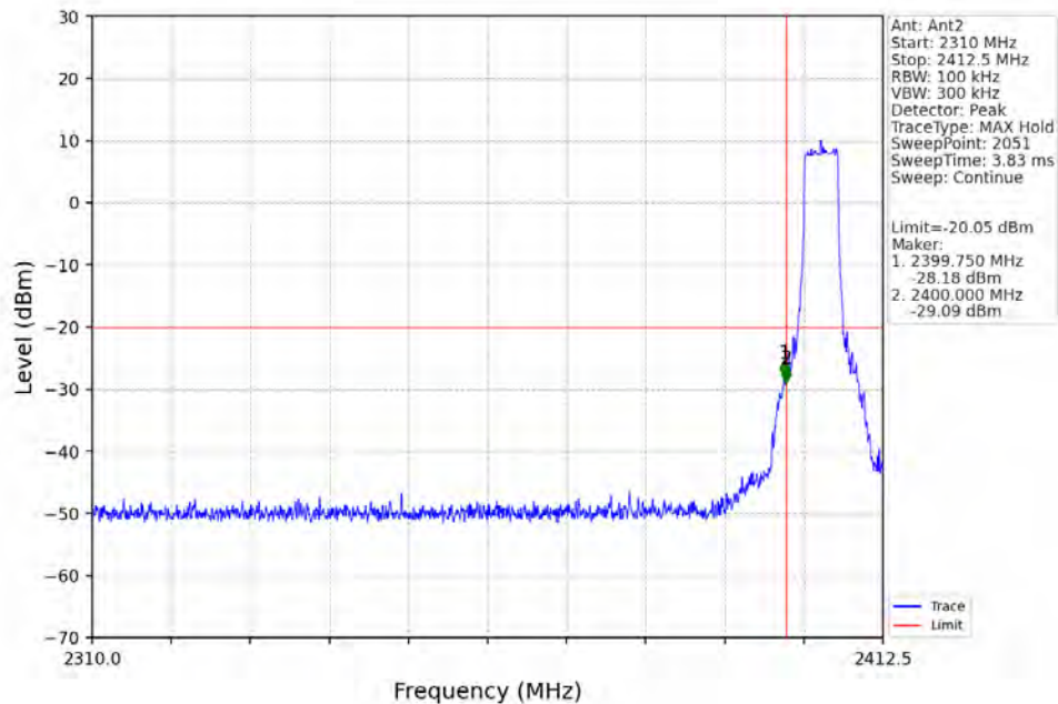
5M_LCH_2404.5MHz_Ant2_NTNV
