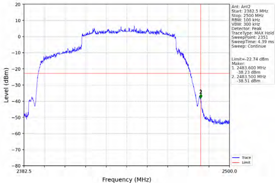
60M_HCH_2442.5MHz_Ant2_NTNV
