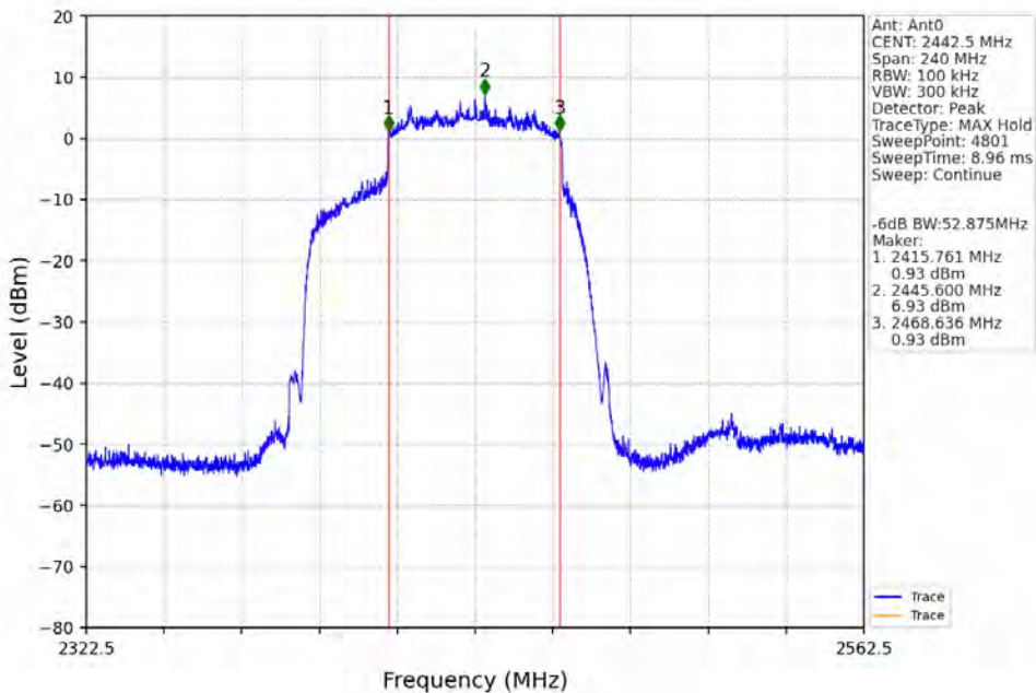
60M_HCH_2442.5MHz_Ant0_NTNV
