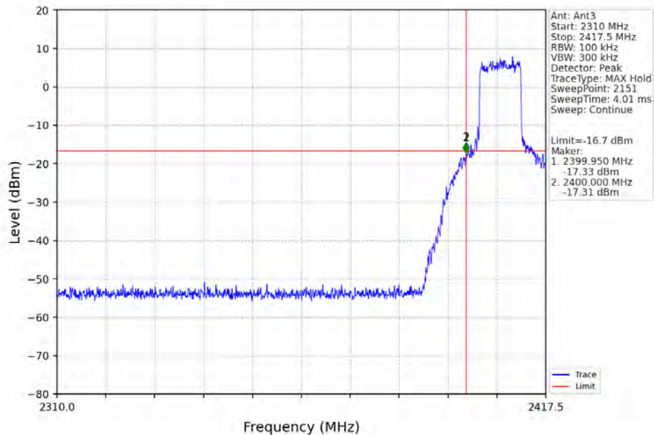
10M_LCH_2407.5MHz_Ant3_NTNV
