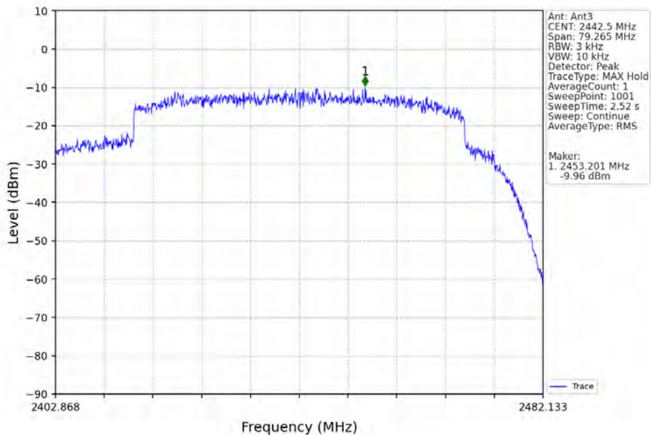
60M_HCH_2442.5MHz_Ant3_NTNV
