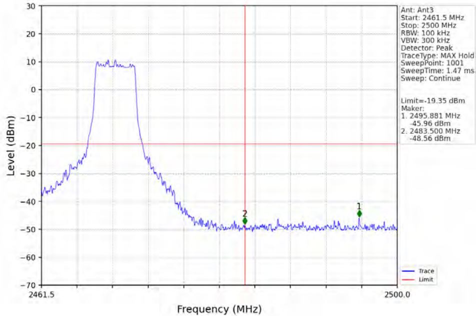
5M_HCH_2469.5MHz_Ant3_NTNV
