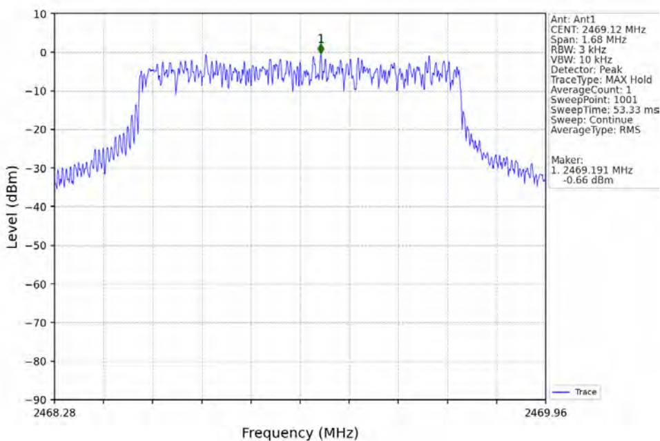
1.4M_HCH_2469.12MHz_Ant1_NTNV
