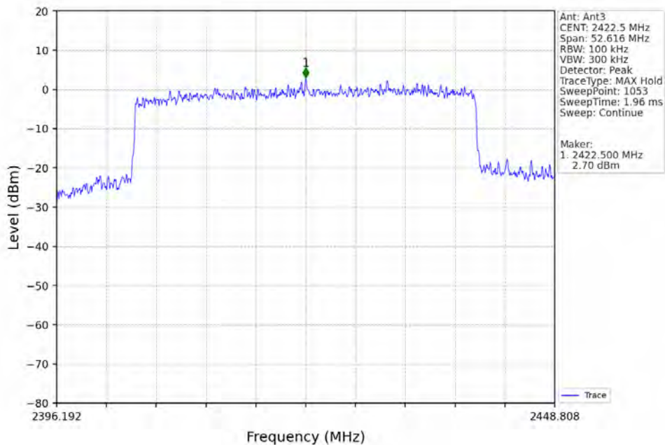
40M_LCH_2422.5MHz_Ant3_NTNV
