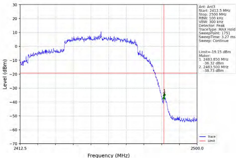
40M_HCH_2452.5MHz_Ant3_NTNV
