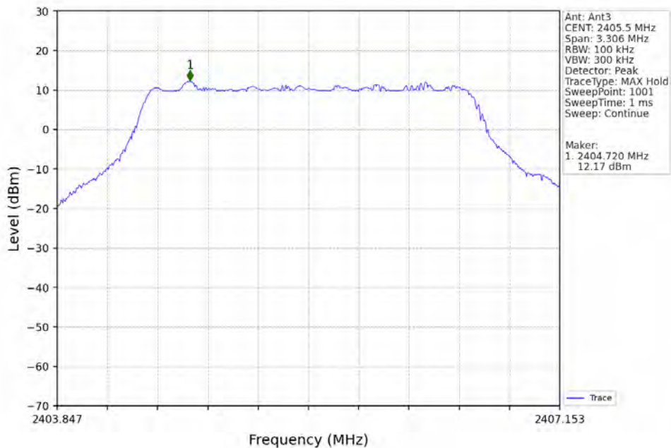
3M_LCH_2405.5MHz_Ant3_NTNV
