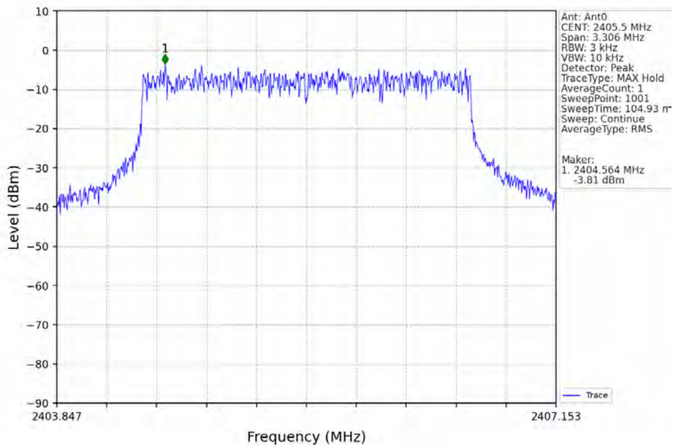
3M_LCH_2405.5MHz_Ant0_NTNV
