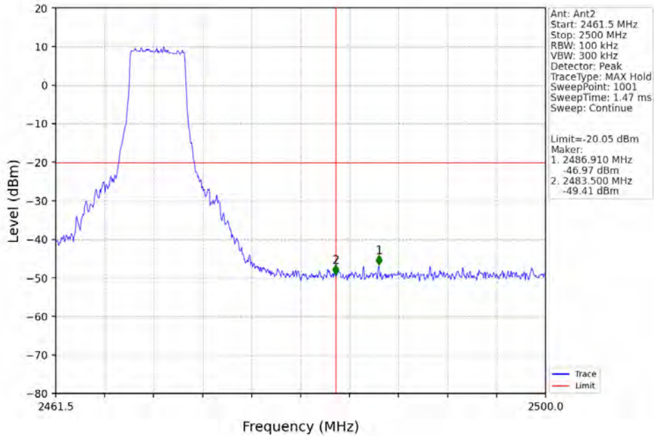
5M_HCH_2469.5MHz_Ant2_NTNV
