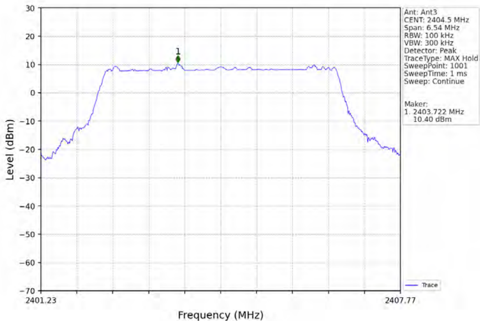
5M_LCH_2404.5MHz_Ant3_NTNV
