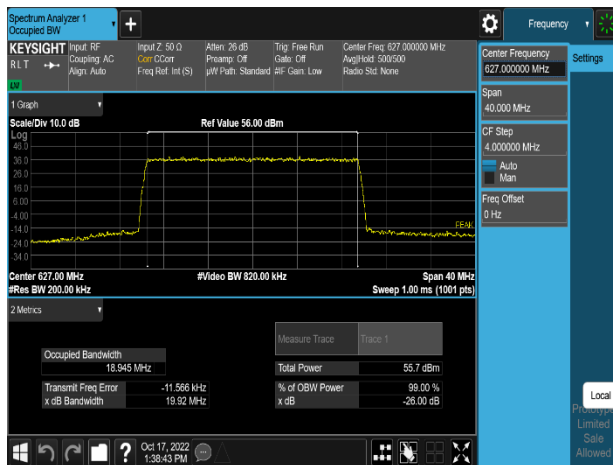
Plot 8-9. Occupied Bandwidth Plot (n71_1C_20M_QPSK - Low Channel, Port 2)
