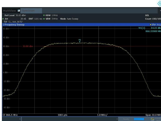
Plot 8-35. Power Spectral Density Plot (n26_1C_5M_16QAM - Mid Channel, Port 2)
