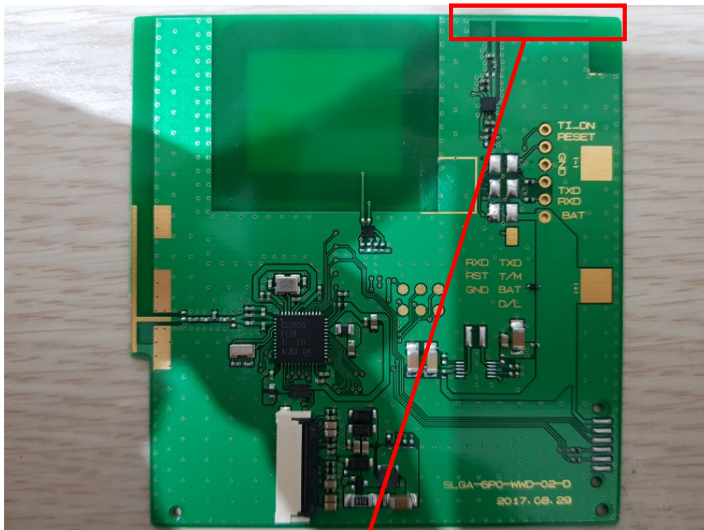
Zigbee receiving Antenna (Wake Up)
