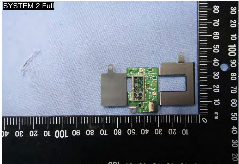
EUT Photo (32)
