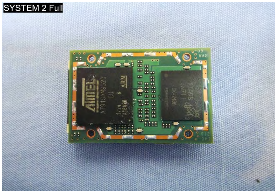
EUT Photo (68)
