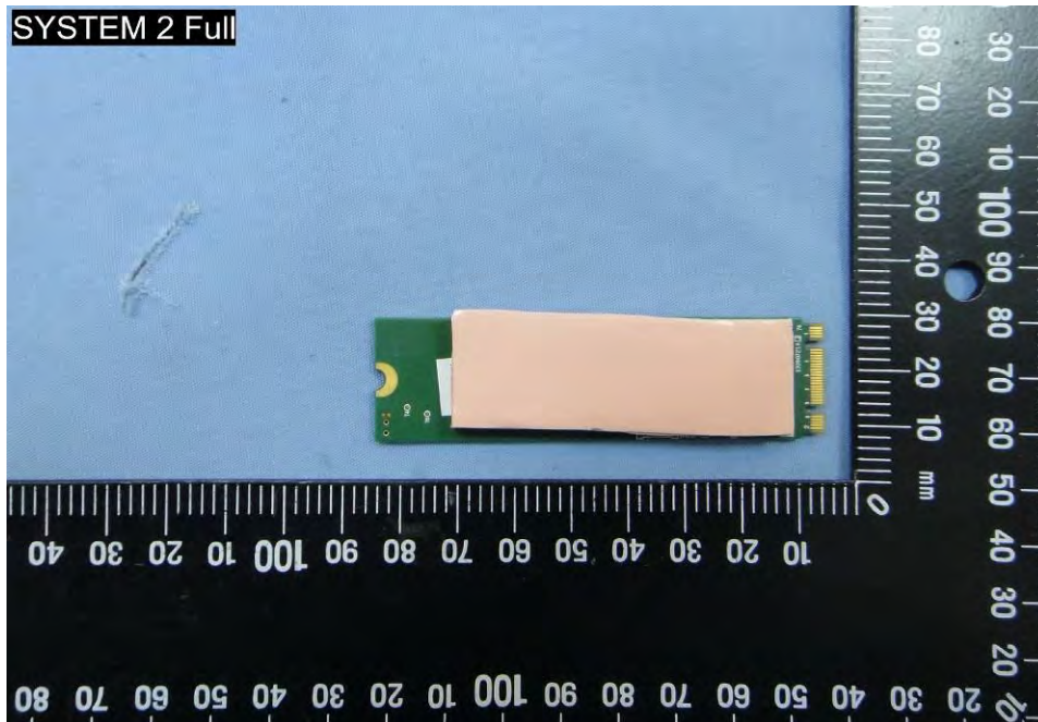
EUT Photo (28)
