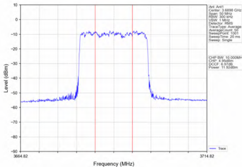
n78d_30kHz_SISO_NTNV_20MHz_DFT-s-OFDM_256_QAM_3690MHz_Inner_Full
