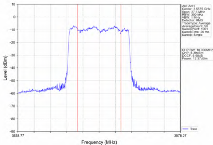
n78d_30kHz_SISO_NTNV_15MHz_CP-OFDM_256_QAM_3557.52MHz_Inner_Full
