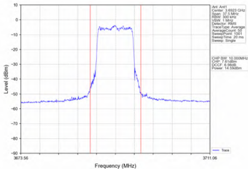
n78d_30kHz_SISO_NTNV_15MHz_CP-OFDM 16 QAM 3692.49MHz_Inner_Full
