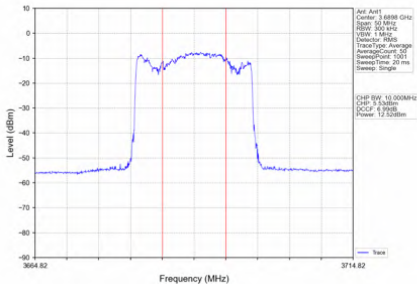
n78d_30kHz_SISO_NTNV_20MHz_DFT-s-OFDM PI/2 BPSK_3690MHz_Inner_Full
