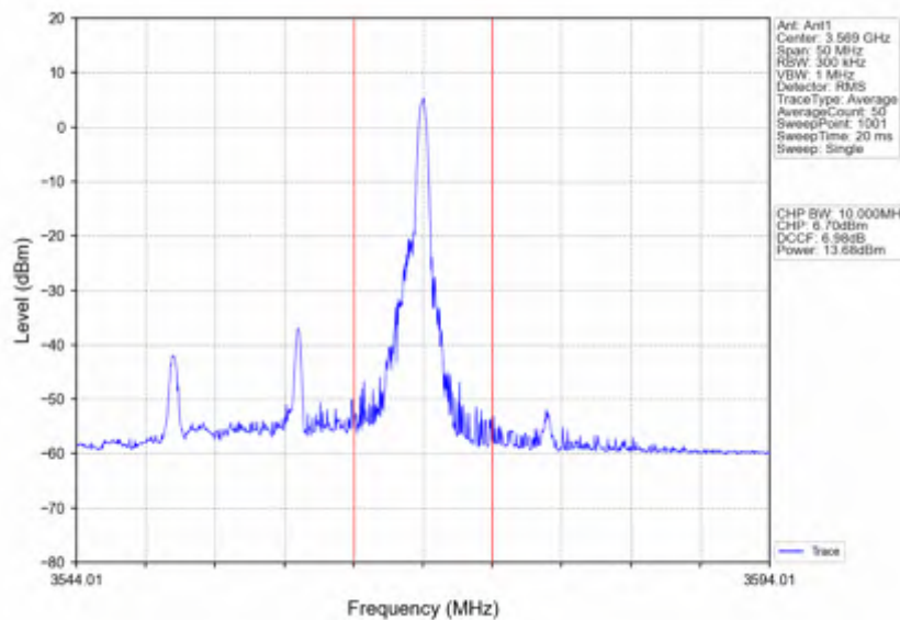
n78d_30kHz_SISO_NTNV_20MHz_CP-OFDM_64_QAM_3560.01MHz_Edge_1RB_Right
