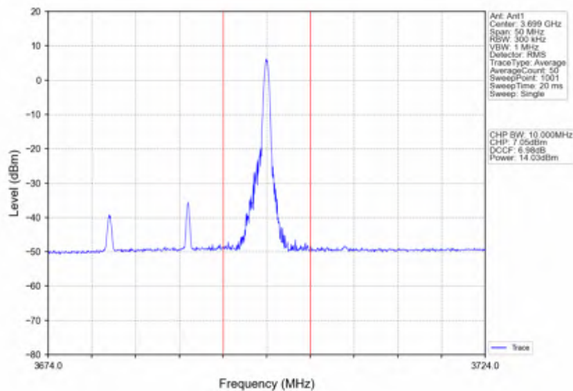
n78d_30kHz_SISO_NTNV_20MHz_CP-OFDM QPSK_3690MHz_Edge_1RB_Right
