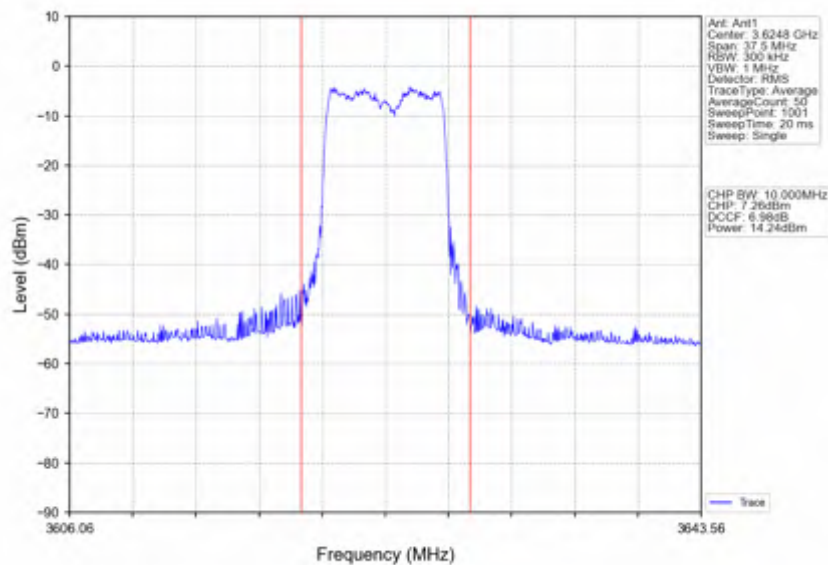
n78d_30kHz_SISO_NTNV_15MHz_CP-OFDM QPSK_3624.99MHz_Inner_Full
