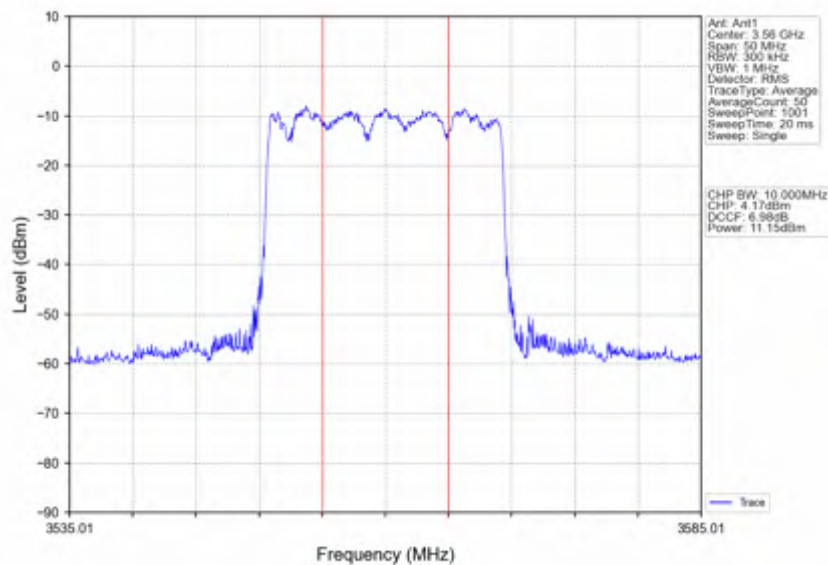
n78d_30kHz_SISO_NTNV_20MHz_CP-OFDM 256 QAM_3560.01MHz_Inner_Full
