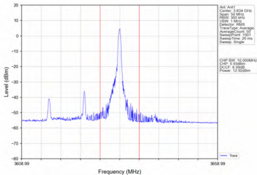
n78d_30kHz_SISO_NTNV_20MHz_DFT-s-OFDM_16_QAM_3624.99MHz_Edge_1RB_Right
