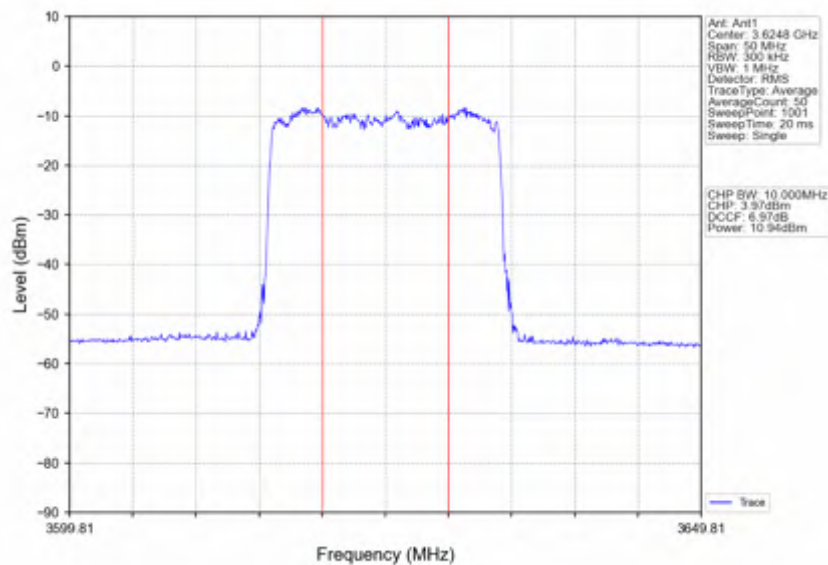
n78d_30kHz_SISO_NTNV_20MHz_DFT-s-OFDM PI/2 BPSK_3624.99MHz_Inner_Full
