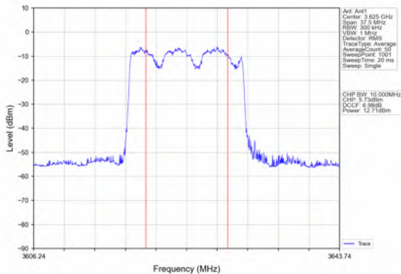
n78d_30kHz_SISO_NTNV_15MHz_CP-OFDM 64 QAM_3624.99MHz_Inner_Full
