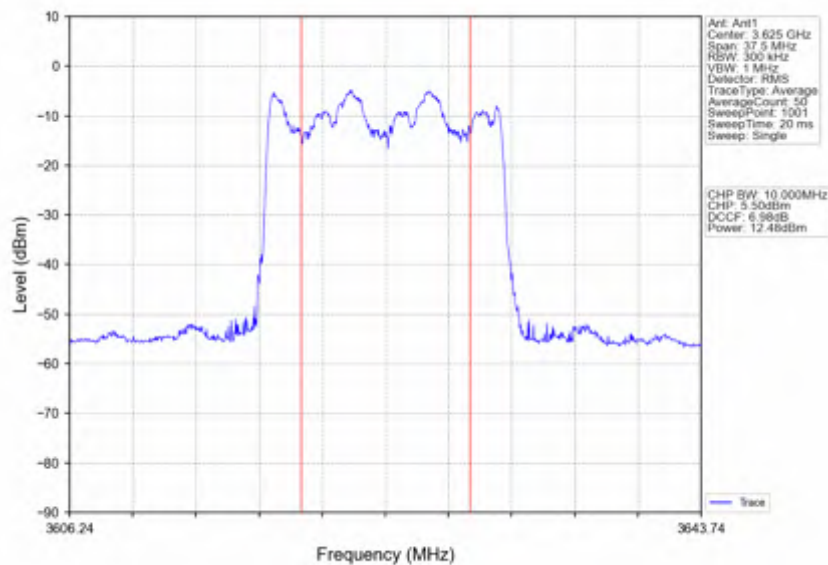
n78d_30kHz_SISO_NTNV_15MHz_CP-OFDM 256 QAM_3624.99MHz_Inner_Full
