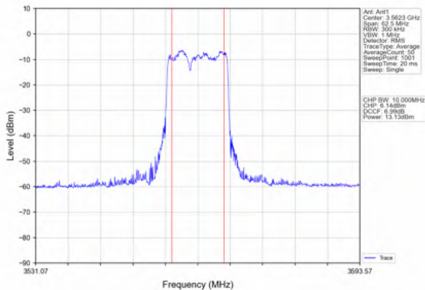
n78d_30kHz_SISO_NTNV_25MHz_DFT-s-OFDM QPSK_3562.5MHz_Inner_Full
