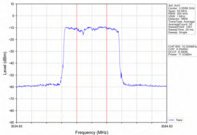
n78d_30kHz_SISO_NTNV_20MHz_DFT-s-OFDM PI/2 BPSK_3560.01MHz_Inner_Full
