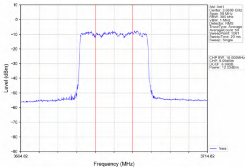
n78d_30kHz_SISO_NTNV_20MHz_DFT-s-OFDM 64 QAM_3690MHz_Inner_Full
