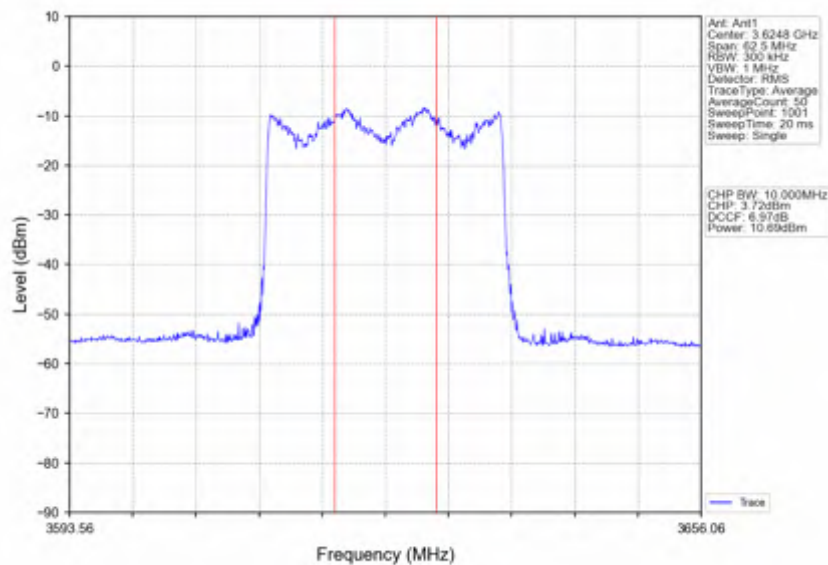
n78d_30kHz_SISO_NTNV_25MHz_DFT-s-OFDM_QPSK_3624.99MHz_Inner_Full
