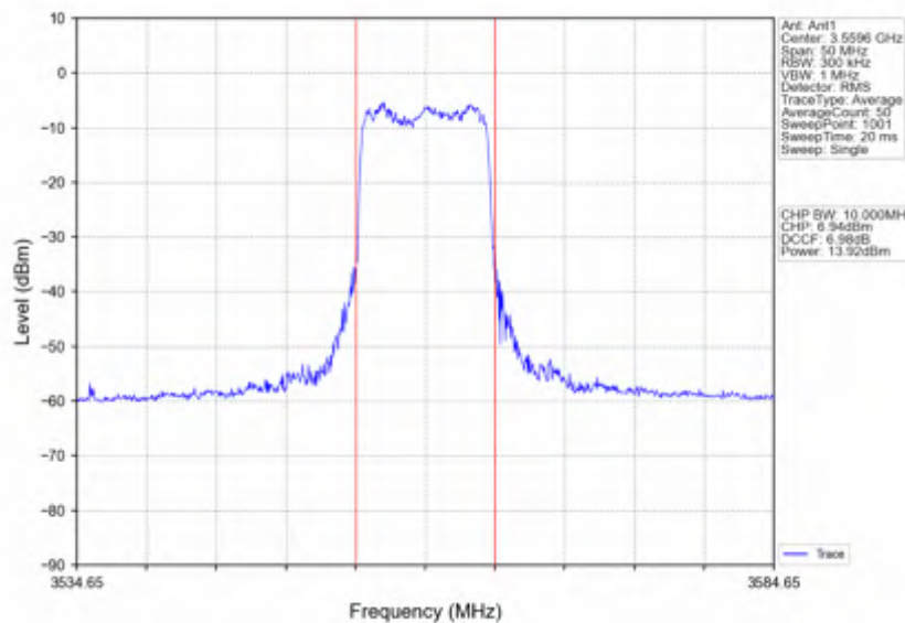
n78d_30kHz_SISO_NTNV_20MHz_CP-OFDM 16 QAM_3560.01MHz_Inner_Full
