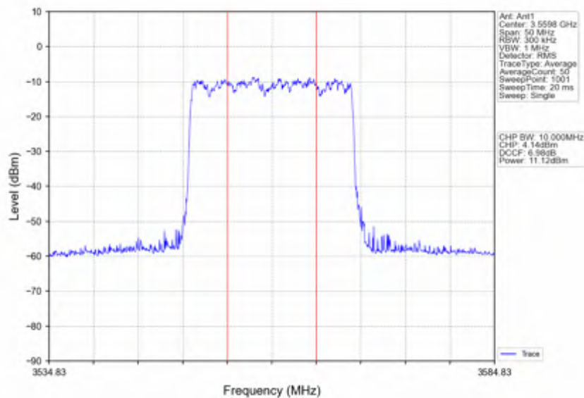
n78d_30kHz_SISO_NTNV_20MHz_DFT-s-OFDM_QPSK_3560.01MHz_Inner_Full
