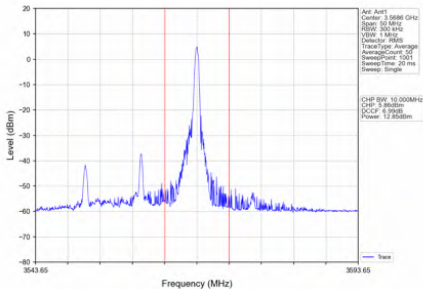
n78d_30kHz_SISO_NTNV_20MHz_DFT-s-OFDM 64 QAM_3560.01MHz_Inner_1RB_Right
