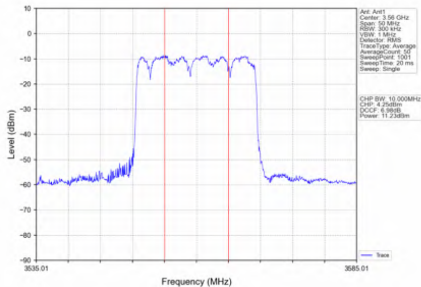
n78d_30kHz_SISO_NTNV_20MHz_CP-OFDM QPSK_3560.01MHz_Inner_Full
