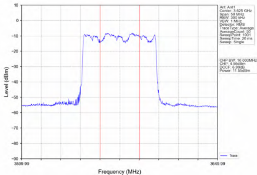
n78d_30kHz_SISO_NTNV_20MHz_CP-OFDM QPSK_3624.99MHz_Inner_Full
