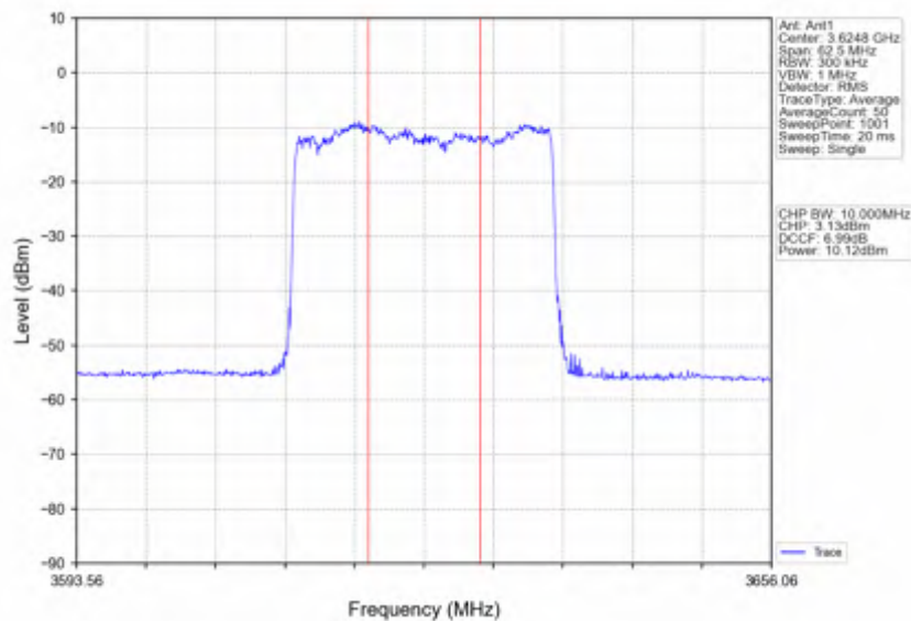
n78d_30kHz_SISO_NTNV_25MHz_DFT-s-OFDM PI/2 BPSK_3624.99MHz_Inner_Full
