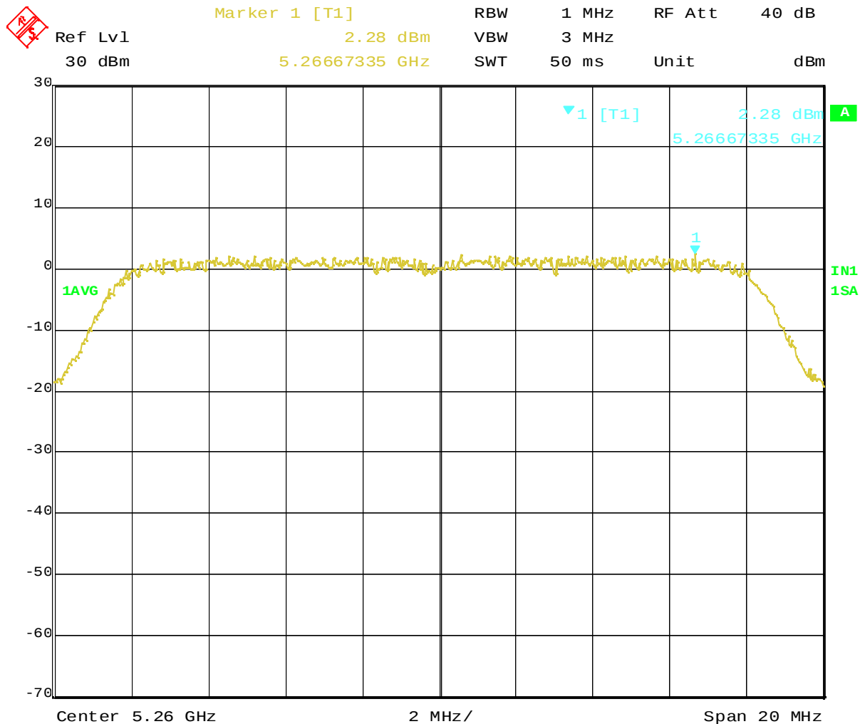
Plot 3-2 Peak Power Spectral Density at 5260MHz
