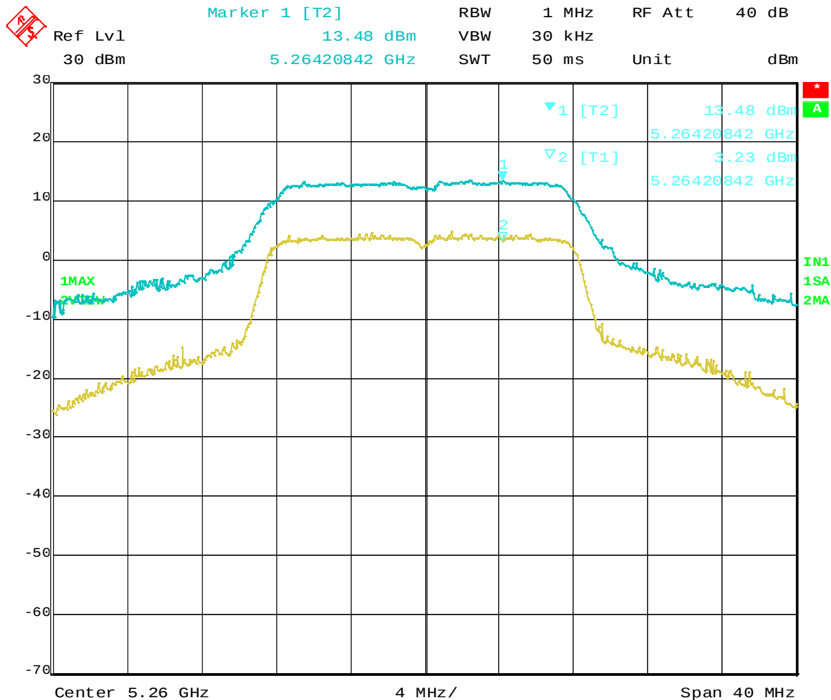
Plot 4-2 Peak Excursion Ratio at 5260MHz
