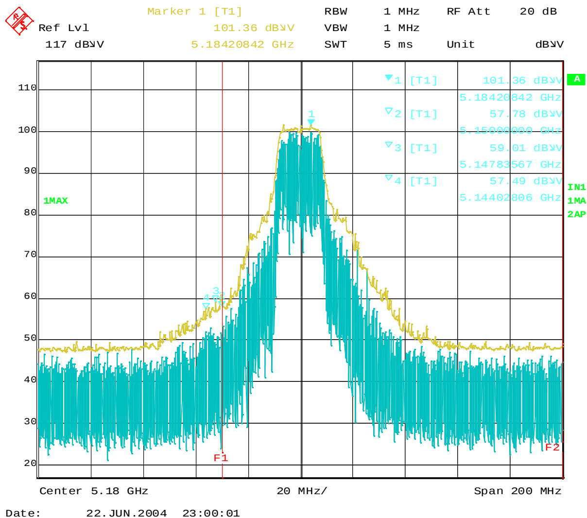
Plot 7-1 5180MHz TX mode (Peak). R50 series
