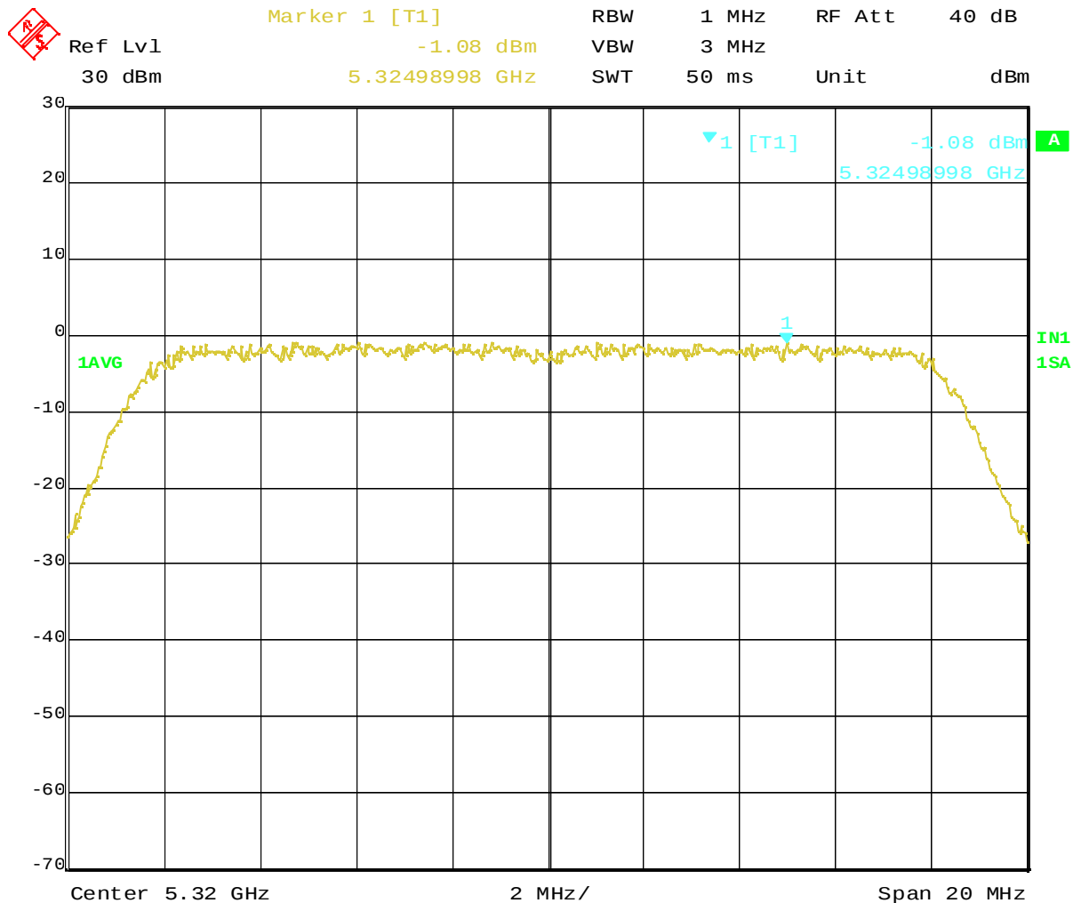
Plot 3-3 Peak Power Spectral Density at 5320MHz
