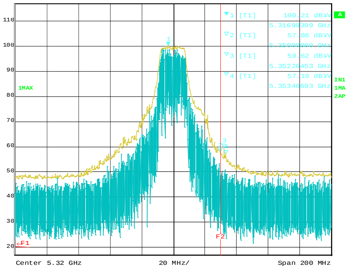
Plot 7-3 5320MHz TX mode (Peak). R50 series
