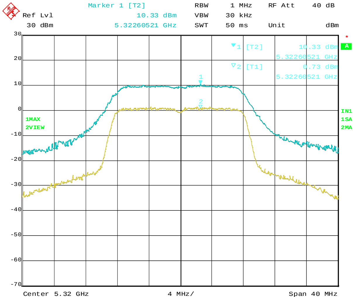
Plot 4-3 Peak Excursion Ratio at 5320MHz
