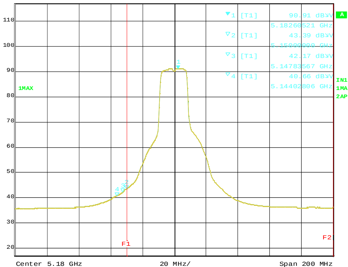
Plot 7-2 5180MHz TX mode (Average). R50 series
