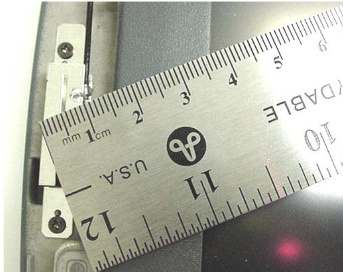
Bluetooth Antenna 3
