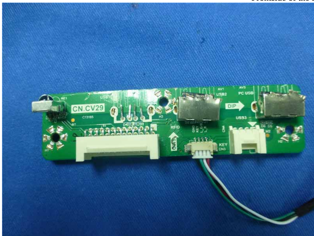
Figure 39 Frontside of the PCB Board
