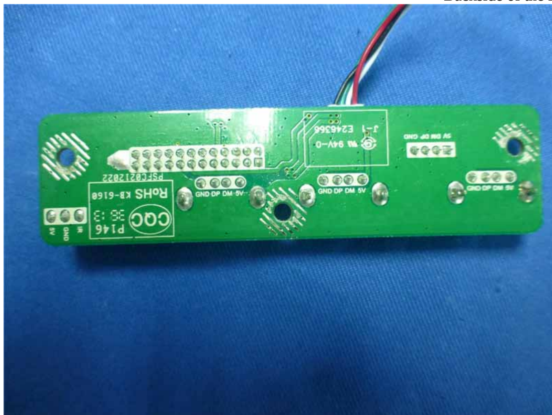
Figure 40 Backside of the PCB Board
