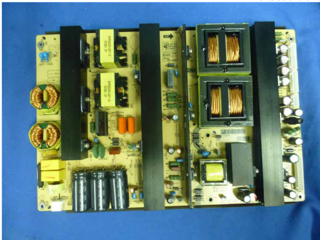
Figure 24 Frontside of the Power Board
