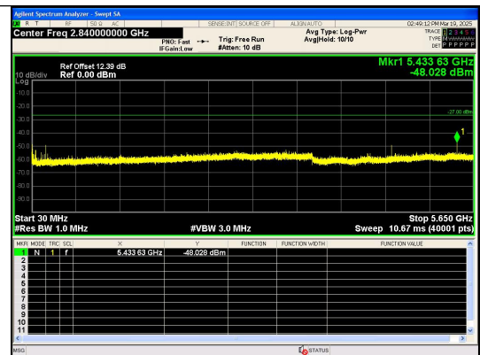
Spurious Emission:30.0~5650 MHz IEEE 802.11ac_Channel 151_40MHz_Antenna 0
