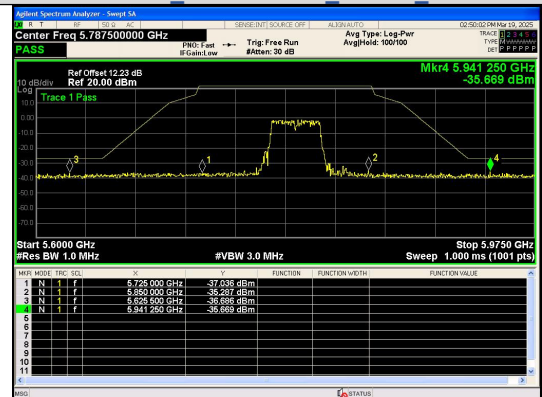
Out Of Band Emission IEEE 802.11ac_Channel 159_40MHz_Antenna 0
