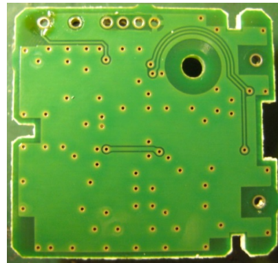
Internal bottom
