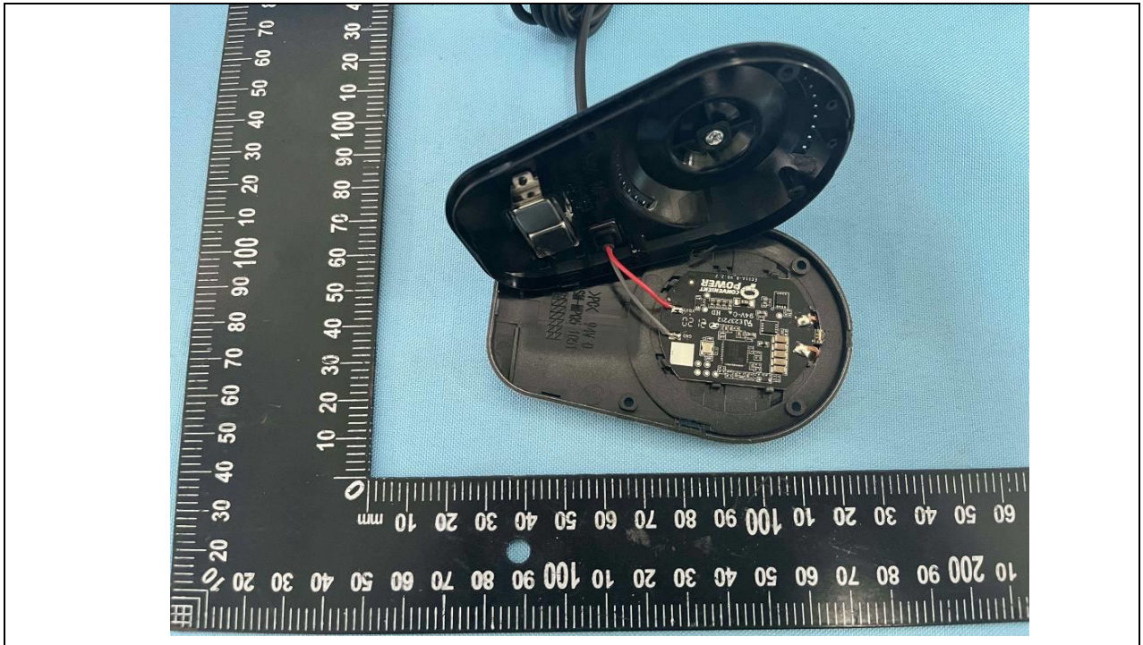
Details of: Wireless charger internal view-4 (Model: MPQ5)
