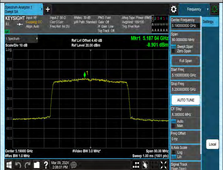
11AX40MIMO-Ant2-5190-PASS
