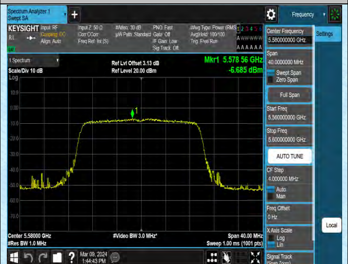
11AX20MIMO-Ant2-5580-PASS
