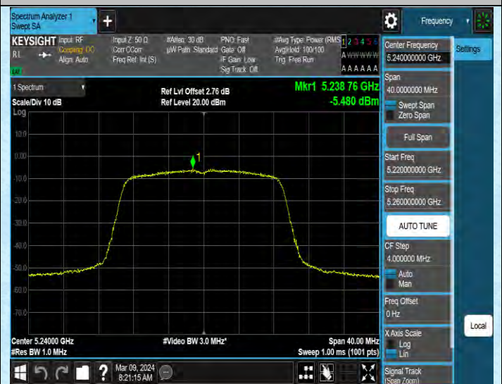
11N20MIMO-Ant2-5240-PASS
