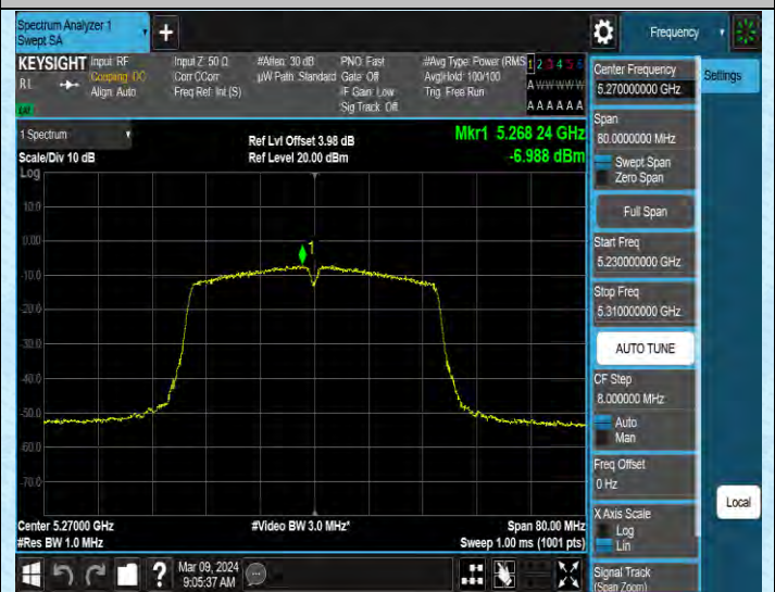
11N40MIMO-Ant2-5270-PASS
