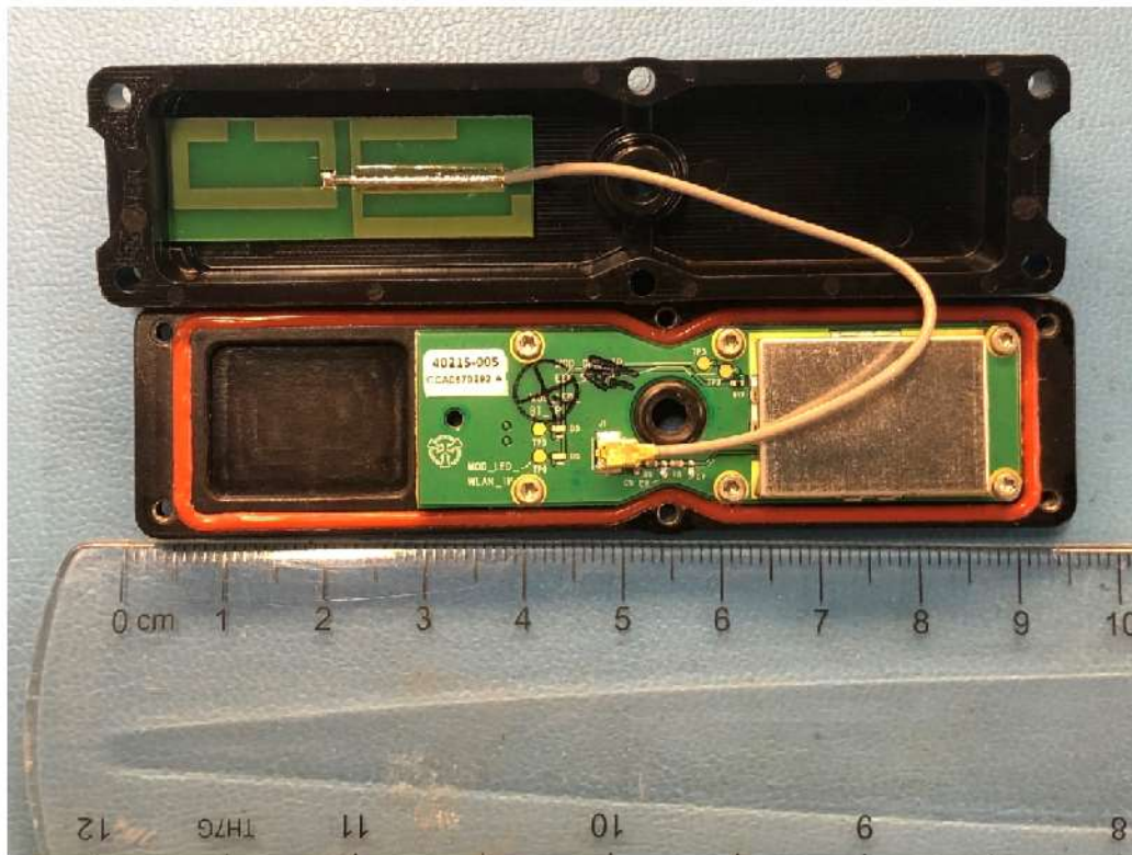
Figure 5: TW-1760, cover open
