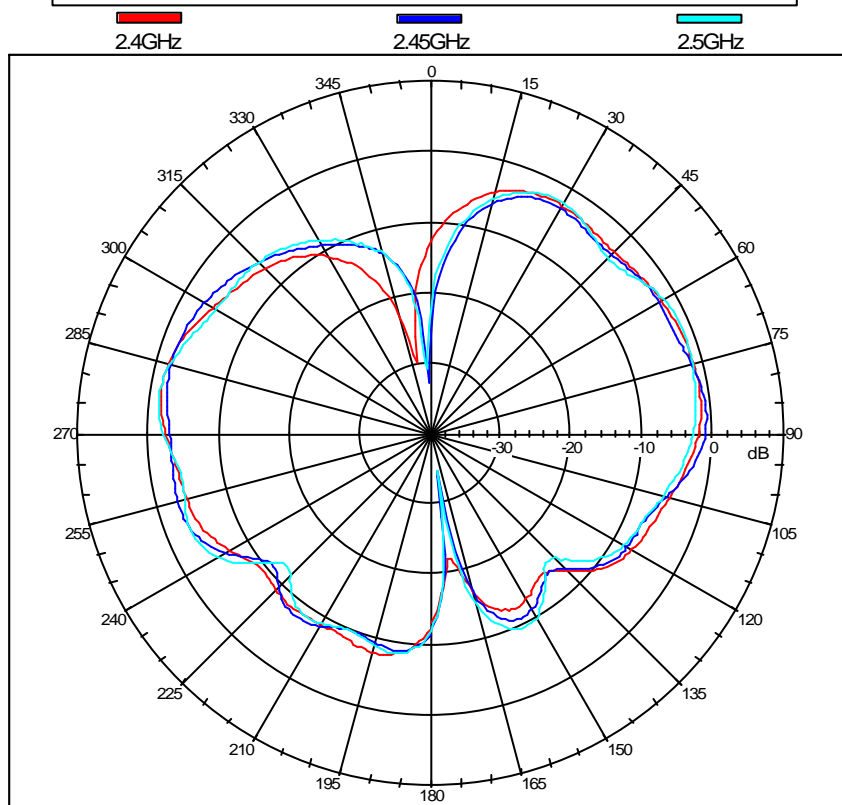
SA3 Dipole Antenna E_Plane
