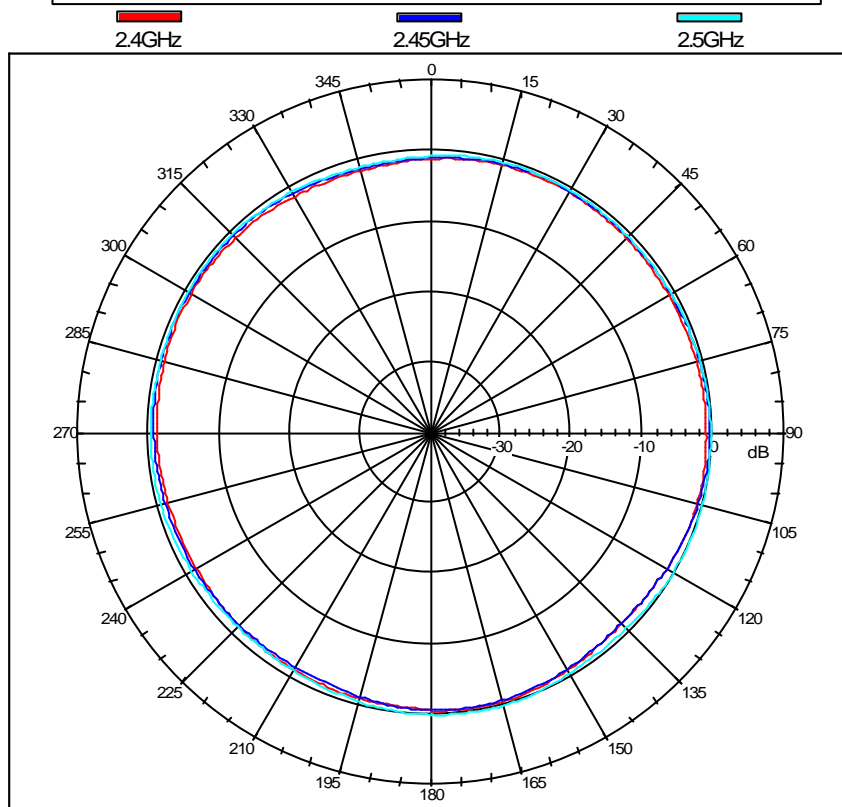
SA3 Dipole Antenna H_Plane
