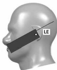
Fig 9.2.1 Handset vertical and horizontal reference lines—"fixed case"
