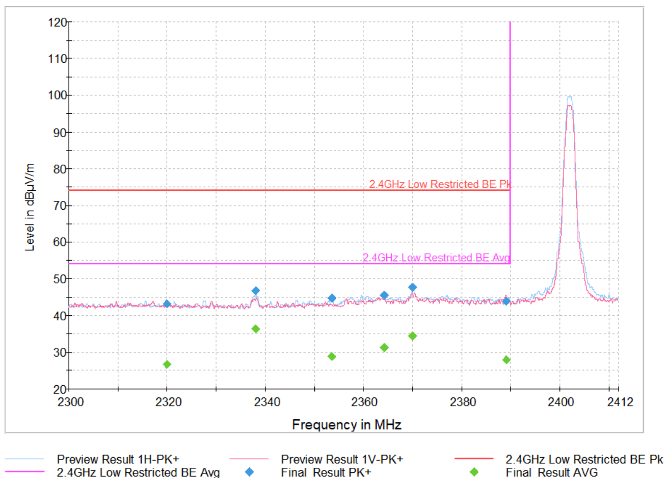
Figure 39: Restricted Band Edge, Low, 2402MHz, 1 Mbps
