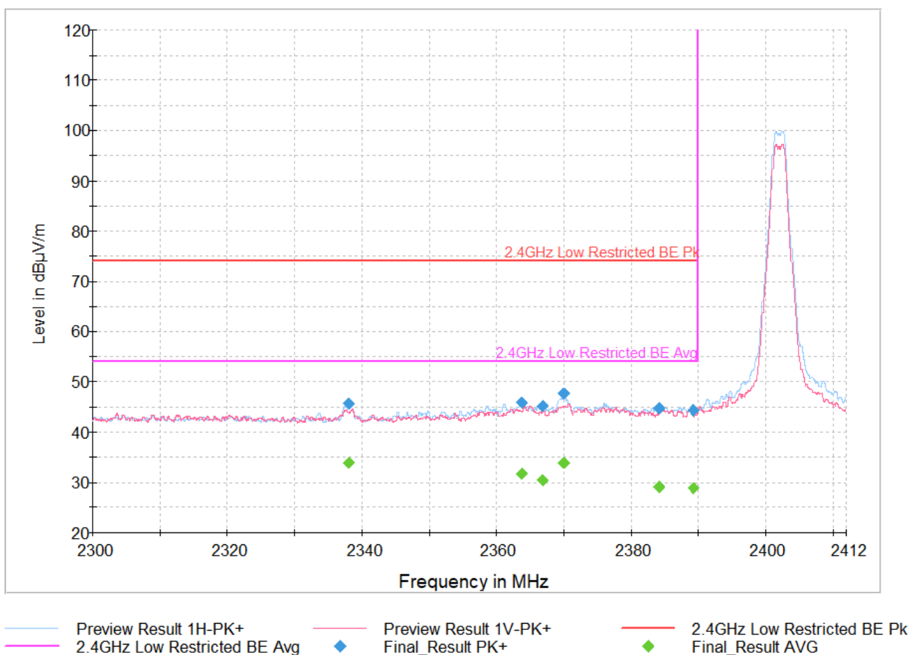
Figure 40: Restricted Band Edge, Low, 2402MHz, 2 Mbps
