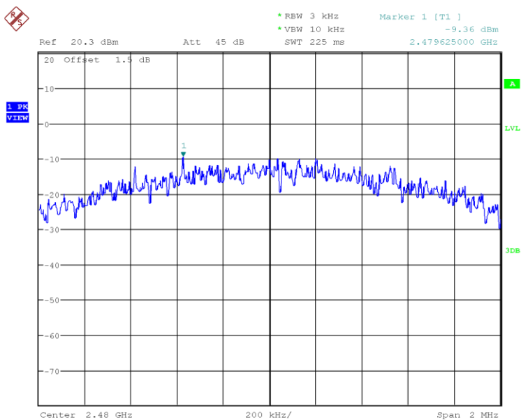
Figure 26: 2480MHz, 2Mbps, PSD
