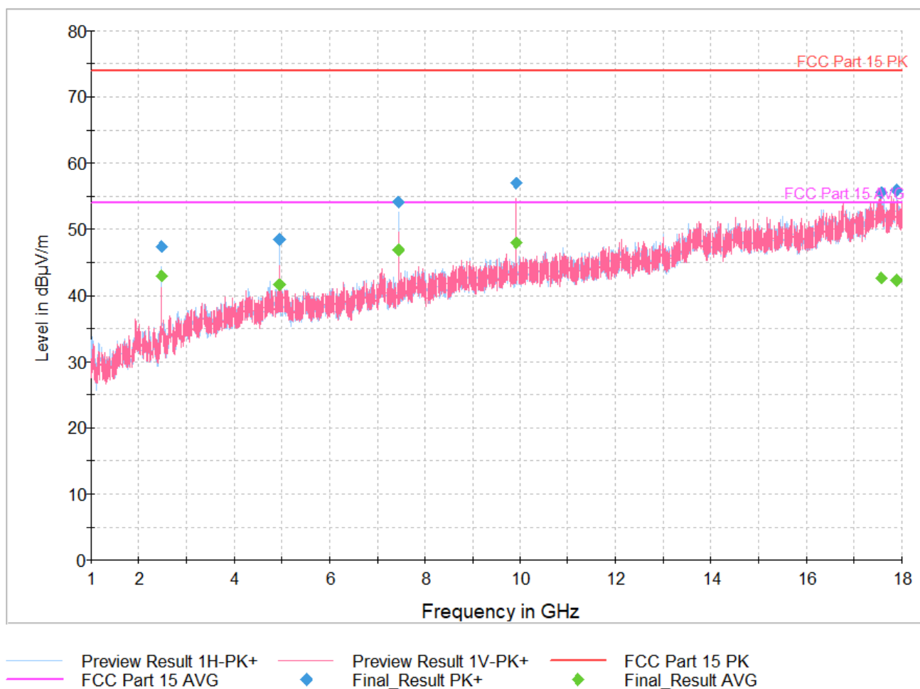
Figure 47: Radiated Spurious Emissions 1GHz - 18GHz, 2480MHz, 1Mbps
