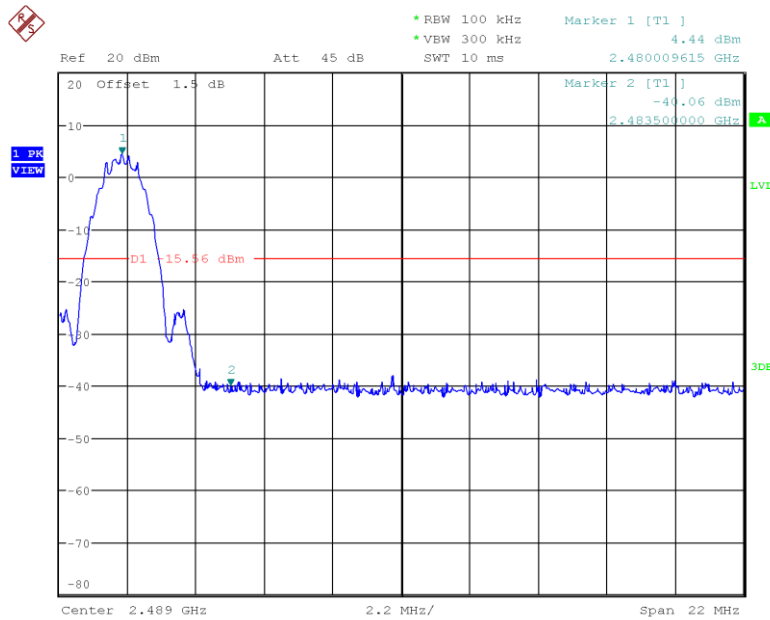
Figure 30: 2480MHz, 2Mbps Upper Band Edge
