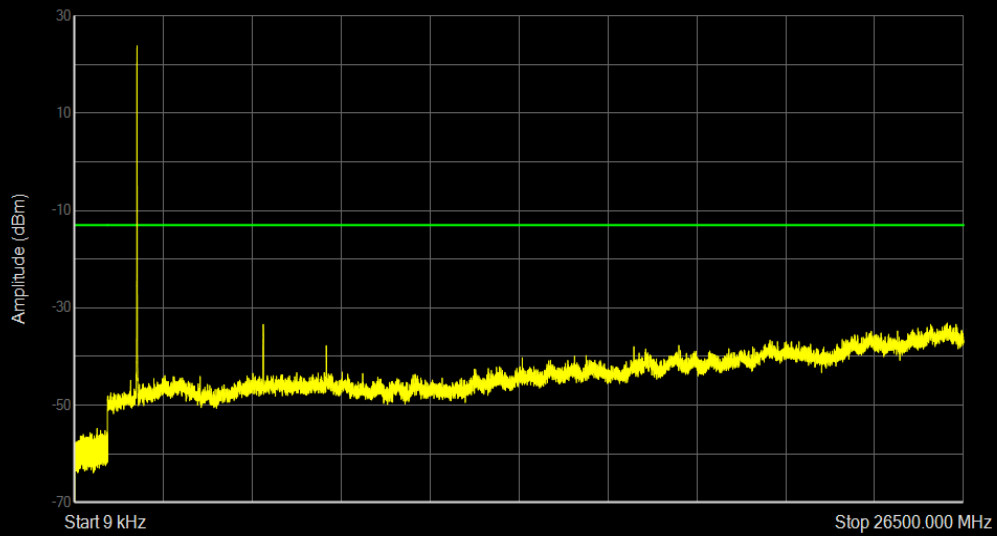
Band2 QAM16 BW=5MHz Channel=18900 RB Size=25 Position=#0
