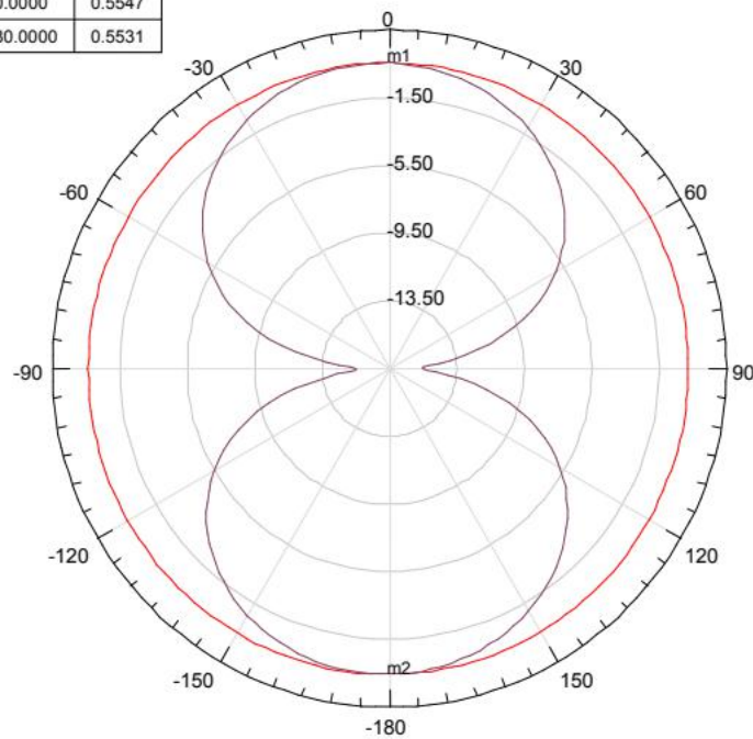
Radiation Patterns(GAIN @ 2440MHz)
