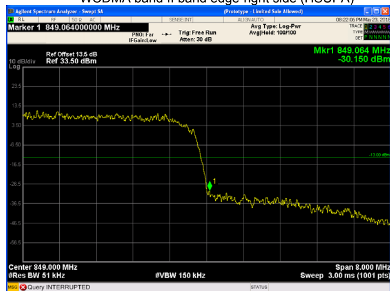
WCDMA band II band edge-right side (HSUPA)
